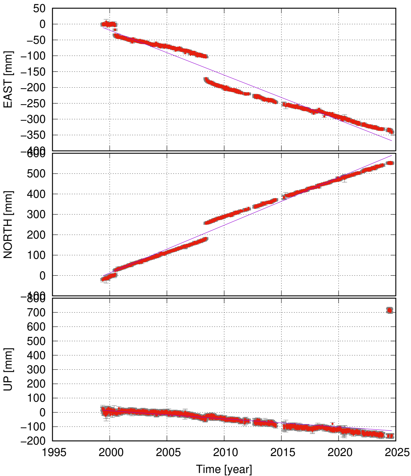
OLKE (64.06, -21.22) time series (ITRF 2014) v_e = -14.15 \pm 0.88 ; v_n = 23.41 \pm 0.89 ; v_u = -5.68 \pm 3.23 mm/yr
