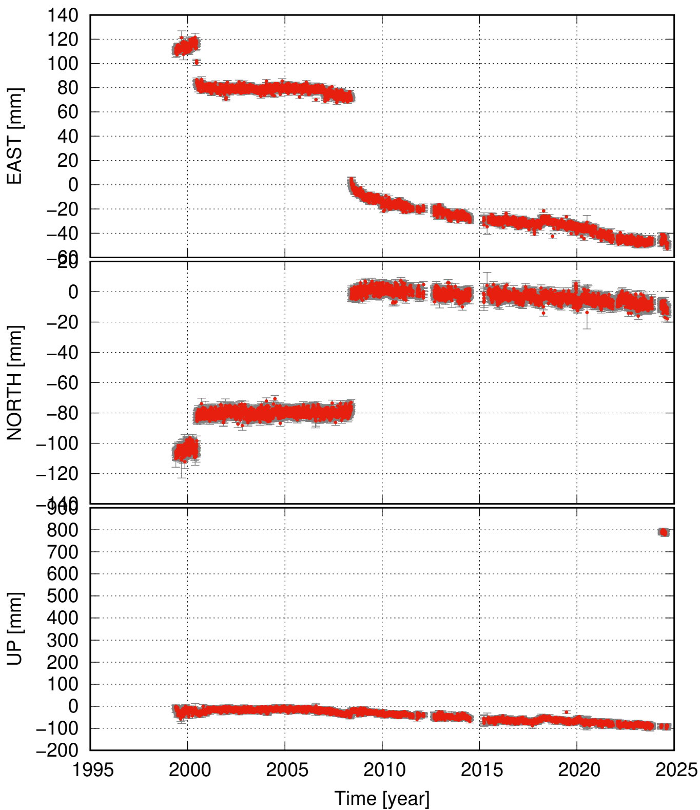
OLKE detrended and seasonal signal removed
