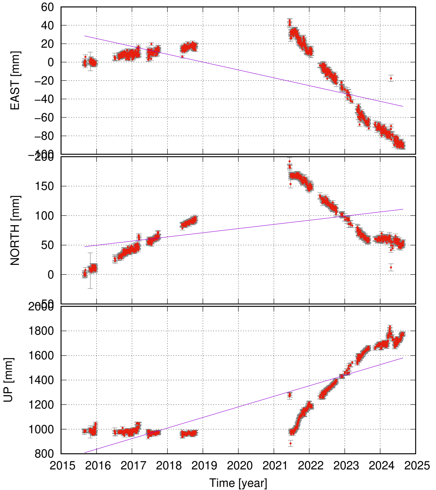
OLAC (65.04, -16.80) time series (ITRF 2014) v_e = -8.53 \pm 3.06 ; v_n = 7.07 \pm 4.61 ; v_u = 85.99 \pm 16.15 mm/yr
