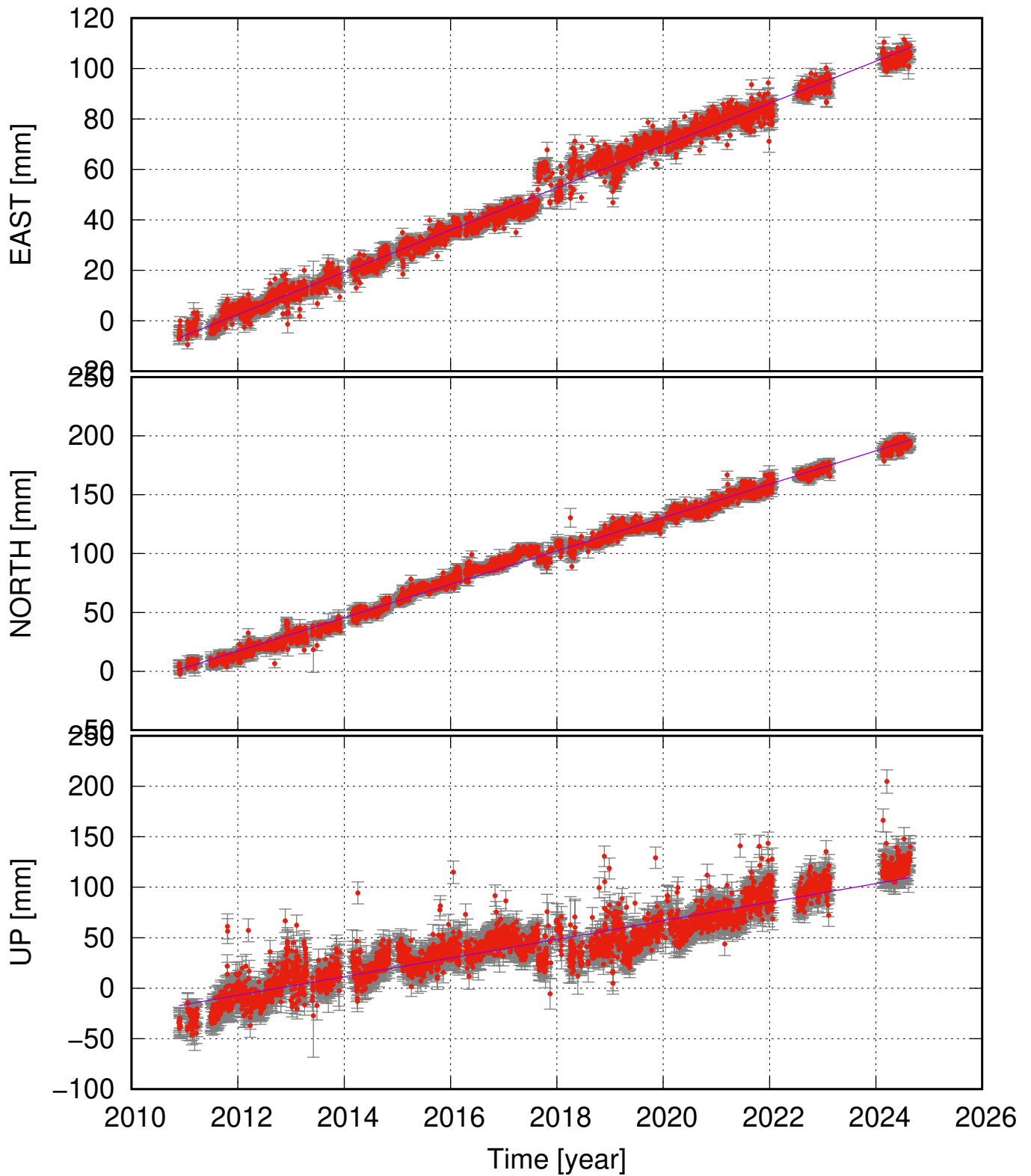
OFEL (63.75, -18.84) time series (ITRF 2014) v_e = 8.37 \pm 0.22 ; v_n = 14.17 \pm 0.32 ; v_u = 9.23 \pm 0.96 mm/yr
