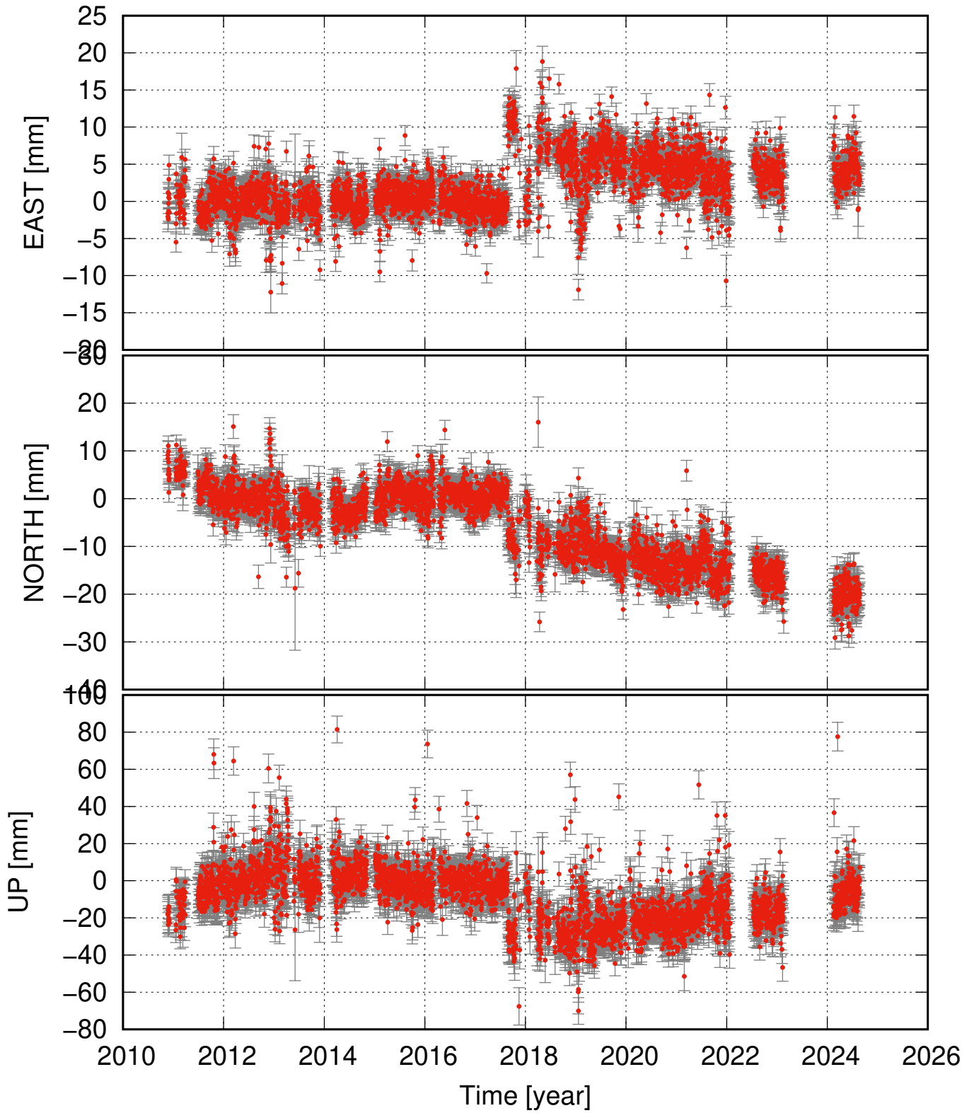
OFEL detrended and seasonal signal removed
