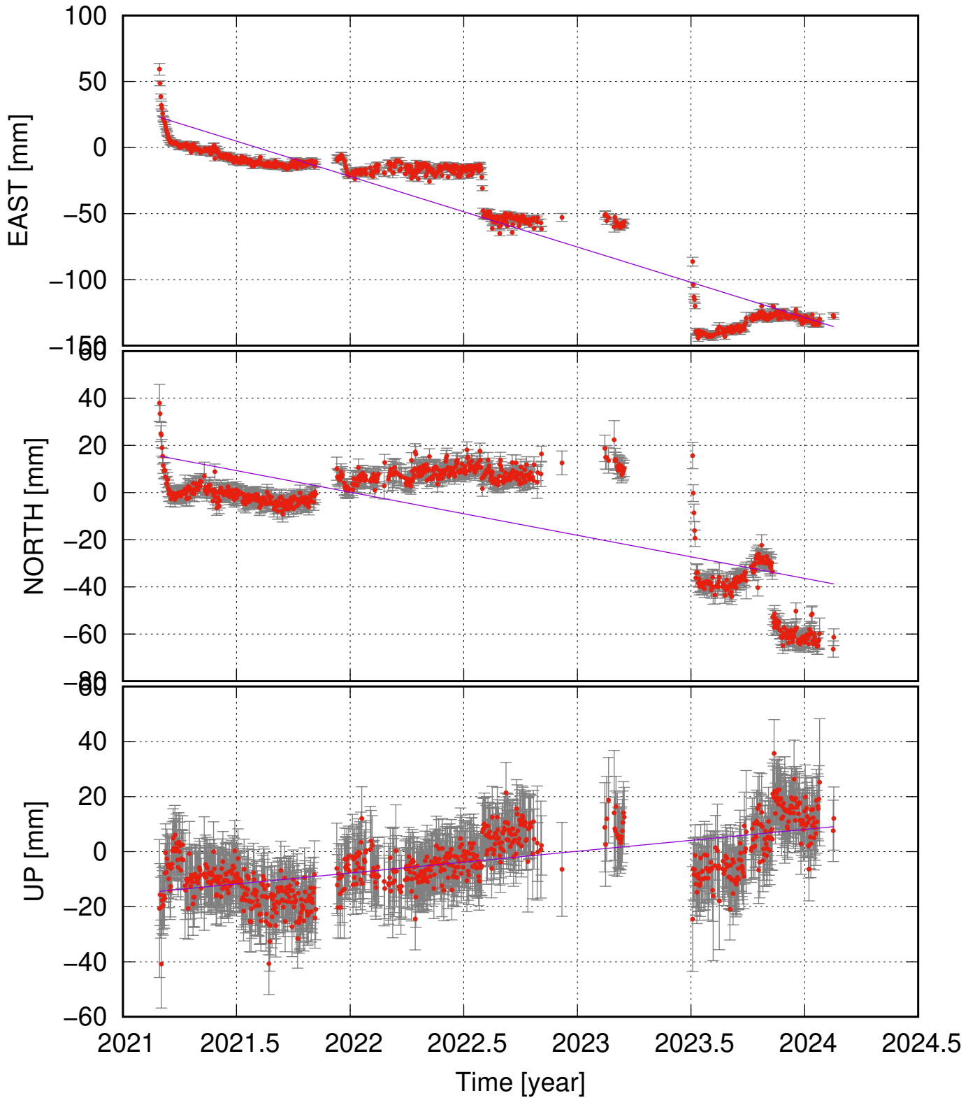
ODDF (63.95, -22.12) time series (ITRF 2014) ve = -53.41 \pm 5.97 ; vn = -18.28 \pm 5.34 ; vu = 7.93 \pm 2.84 mm/yr
