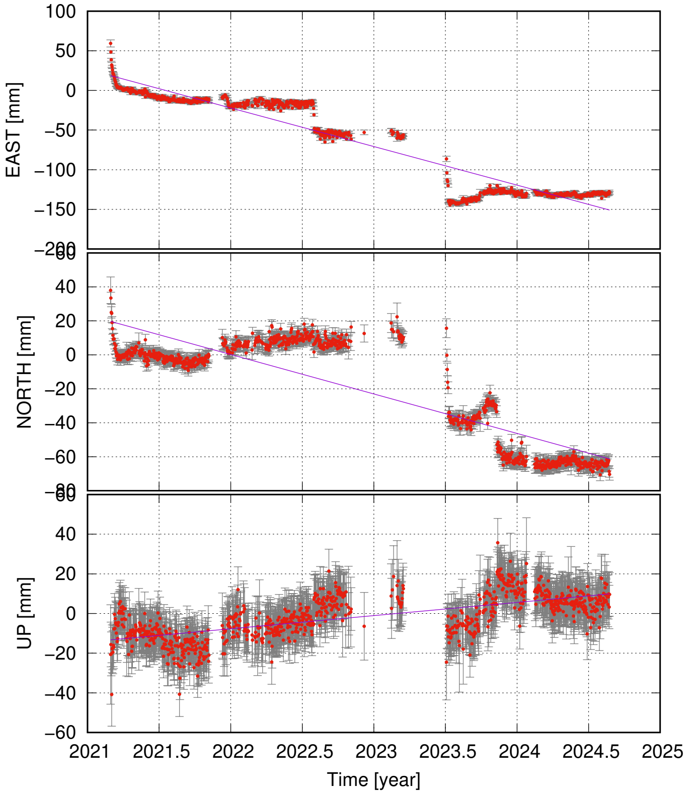
ODDF (63.95, -22.12) time series (ITRF 2014) ve = -48.66 \pm 4.92 ; vn = -23.24 \pm 4.42 ; vu = 6.65 \pm 2.29 mm/yr
