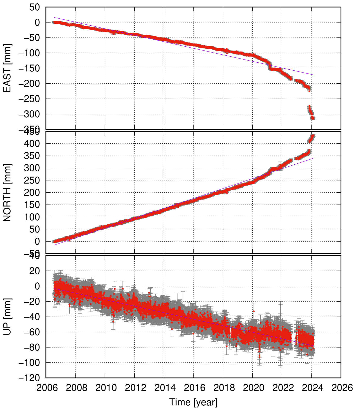
NYLA (63.97, -22.74) time series (ITRF 2014) v_e = -10.69 \pm 1.23 ; v_n = 20.21 \pm 0.85 ; v_u = -4.26 \pm 0.32 mm/yr
