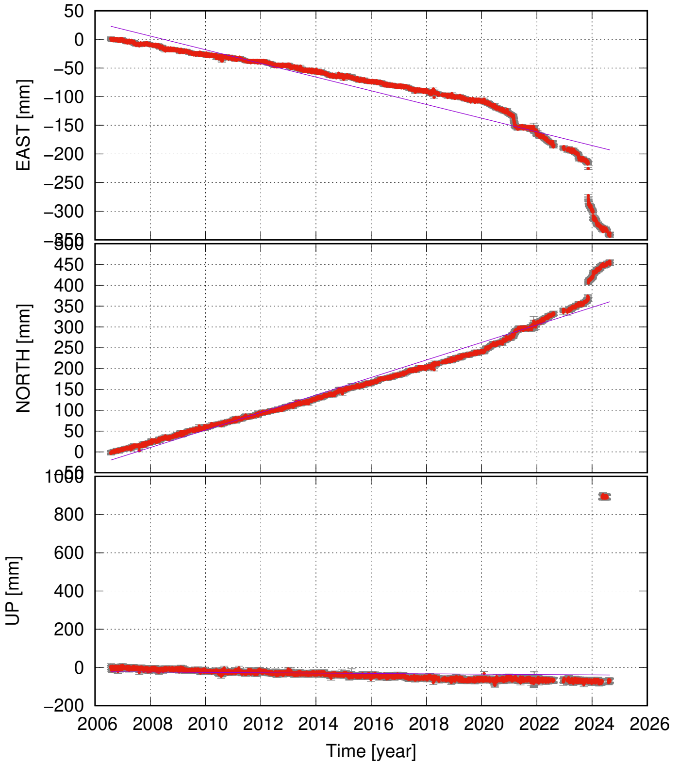
NYLA (63.97, -22.74) time series (ITRF 2014) v_e = -11.95 \pm 1.74 ; v_n = 21.04 \pm 1.17 ; v_u = -0.93 \pm 5.39 mm/yr
