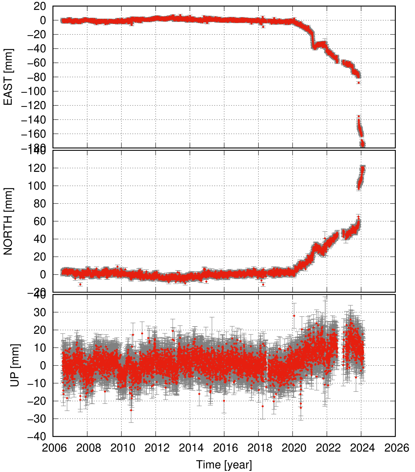
NYLA detrended and seasonal signal removed
