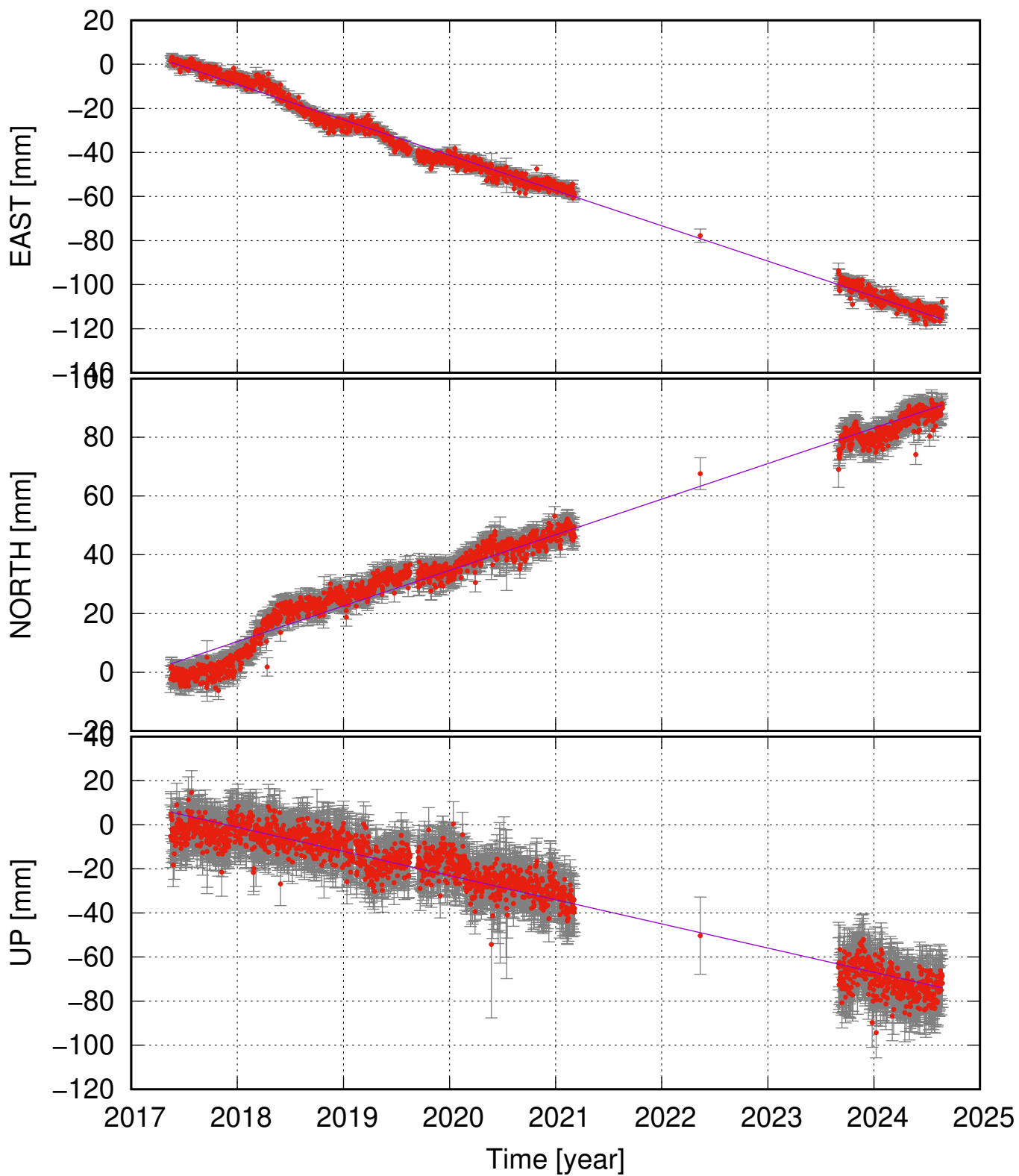
NVEL (64.11, -21.25) time series (ITRF 2014) v_e = -16.03 \pm 0.36 ; v_n = 12.12 \pm 0.55 ; v_u = -10.95 \pm 0.83 mm/yr
