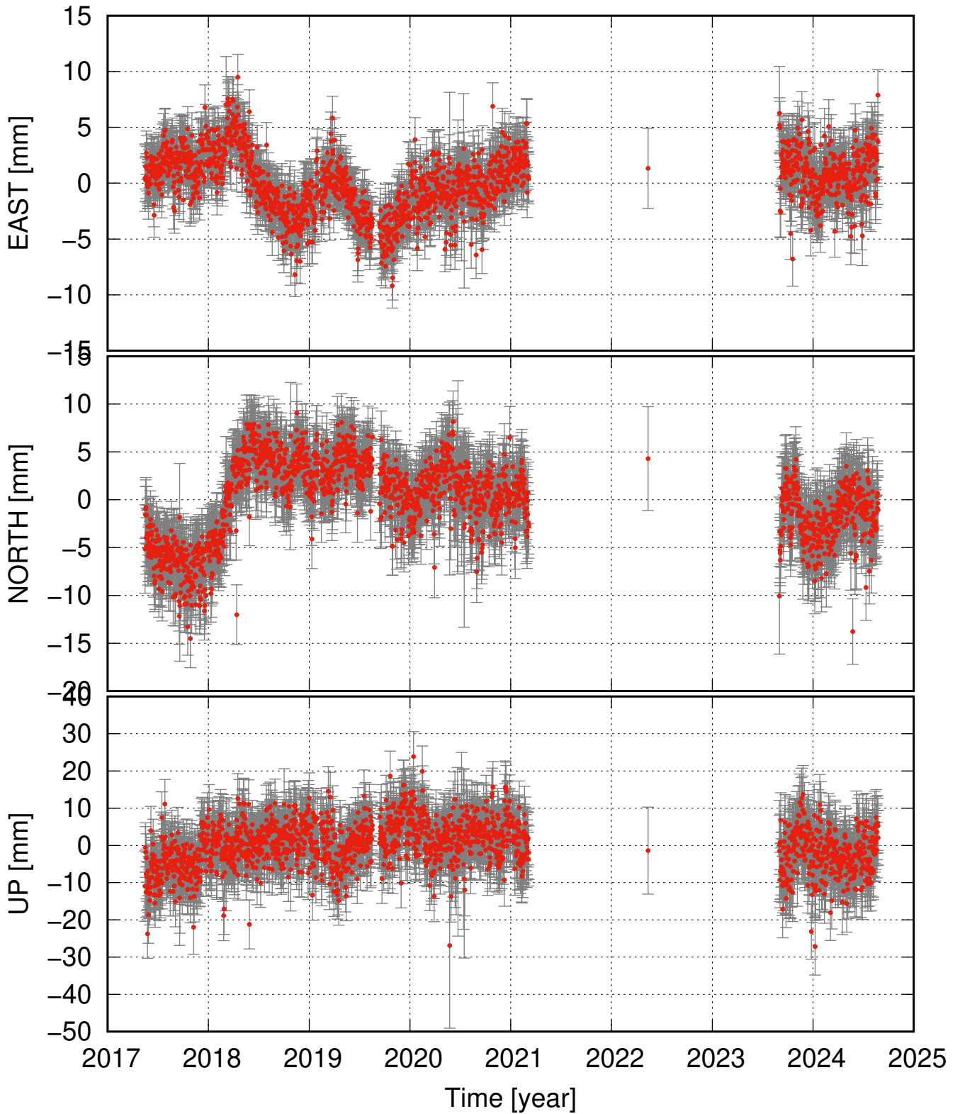
NVEL residual time series (some major events removed as well)
