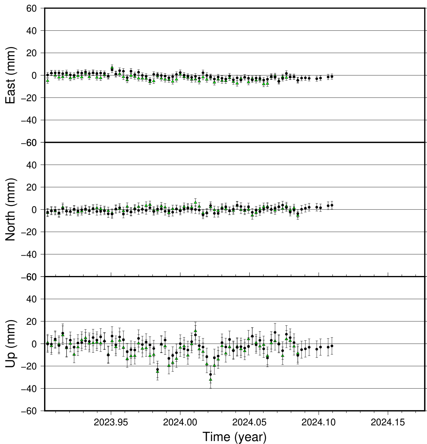
NVEL time series (IGS 2014), last 100 days
