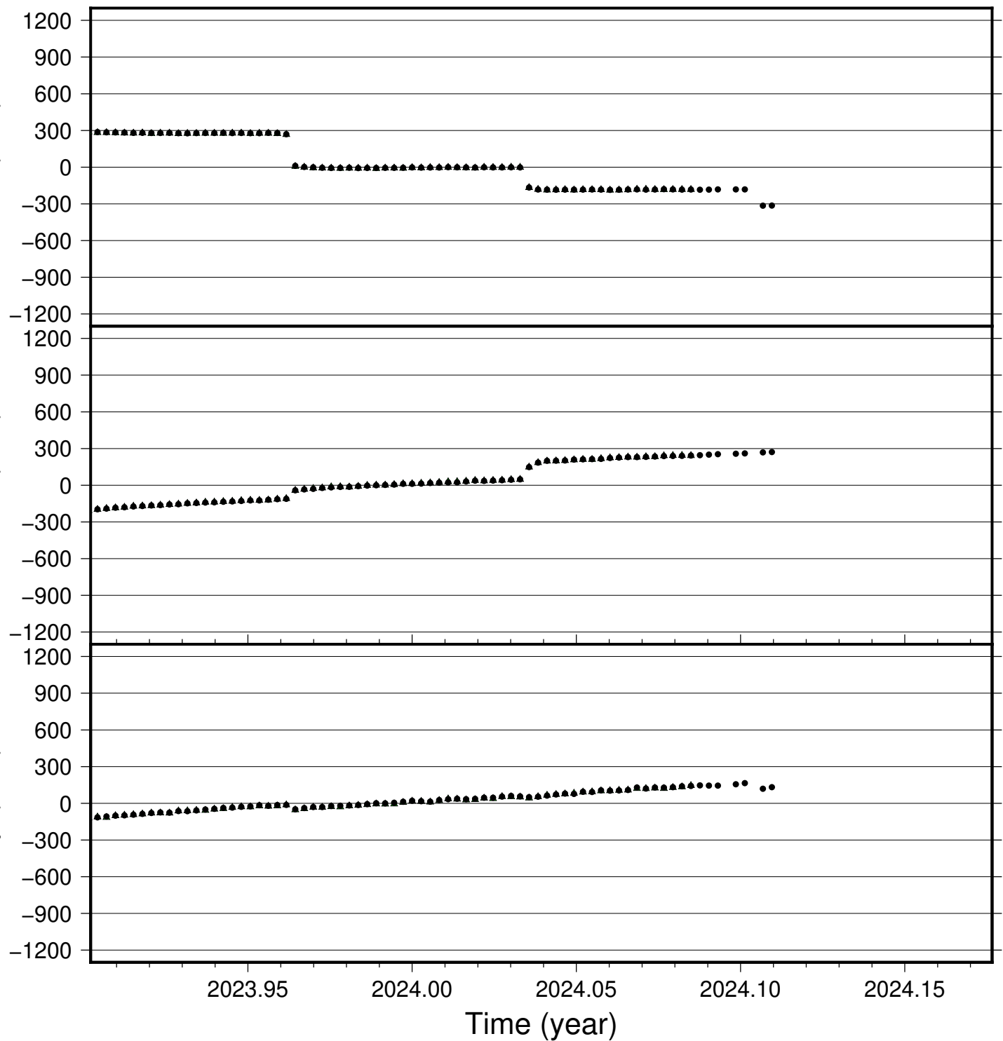
NORV time series (IGS 2014), last 100 days
