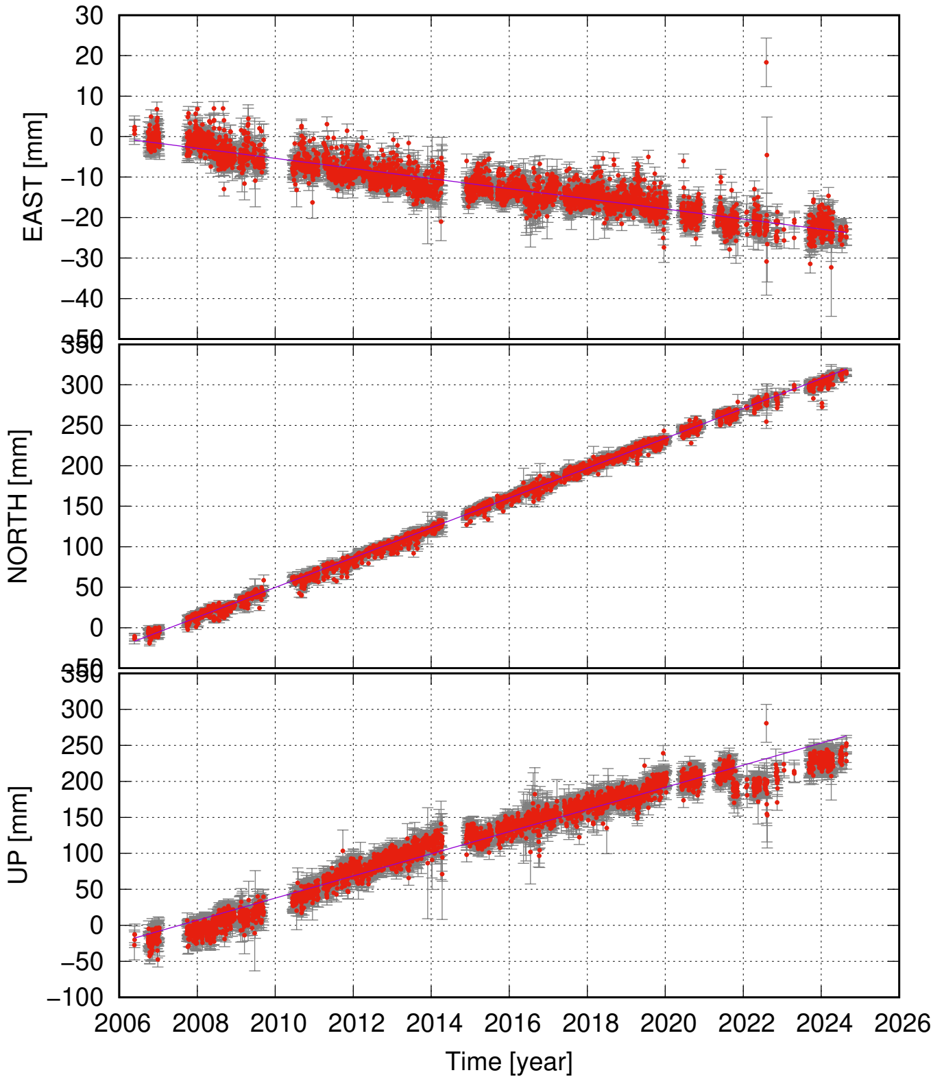
NORS (64.03, -19.72) time series (ITRF 2014) v_e = -1.25 \pm 0.13 ; v_n = 18.42 \pm 0.21 ; v_u = 15.39 \pm 0.76 mm/yr
