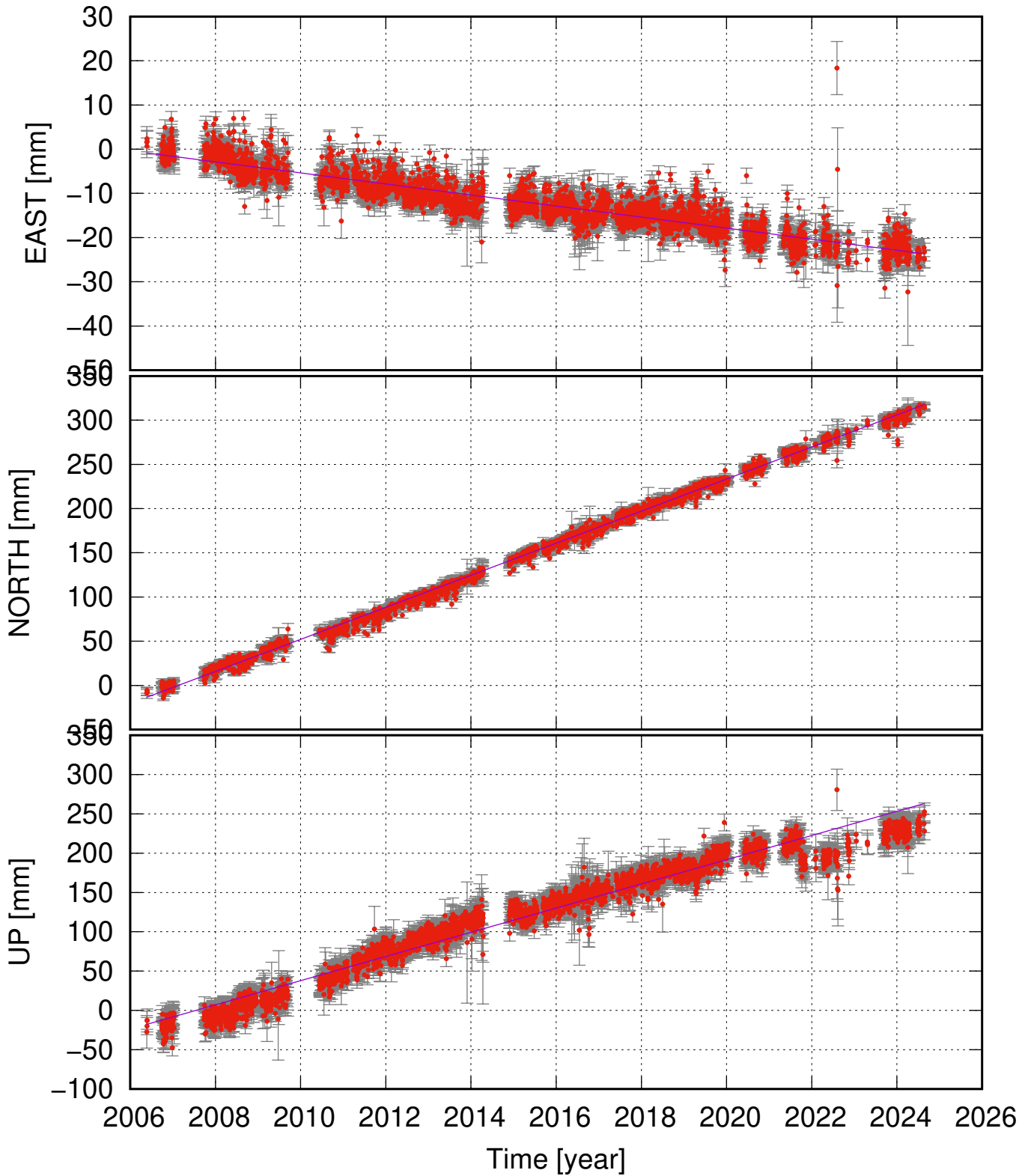
NORS (64.03, -19.72) time series (ITRF 2014) v_e = -1.25 \pm 0.13 ; v_n = 18.14 \pm 0.23 ; v_u = 15.39 \pm 0.76 mm/yr
