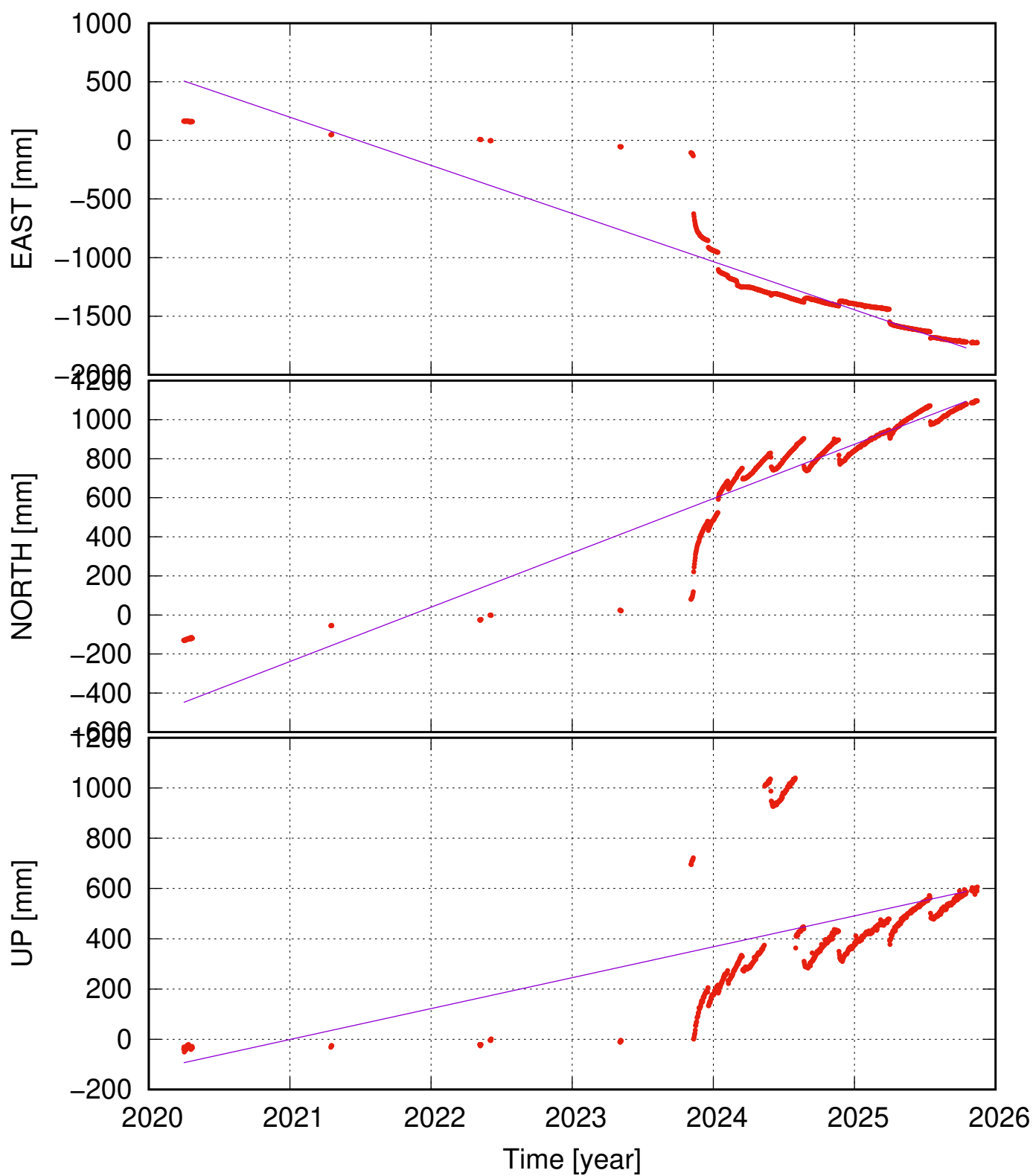
NBIO ( , ) time series (IGb20) ve = +- ; vn = +- ; vu = +- mm/yr
