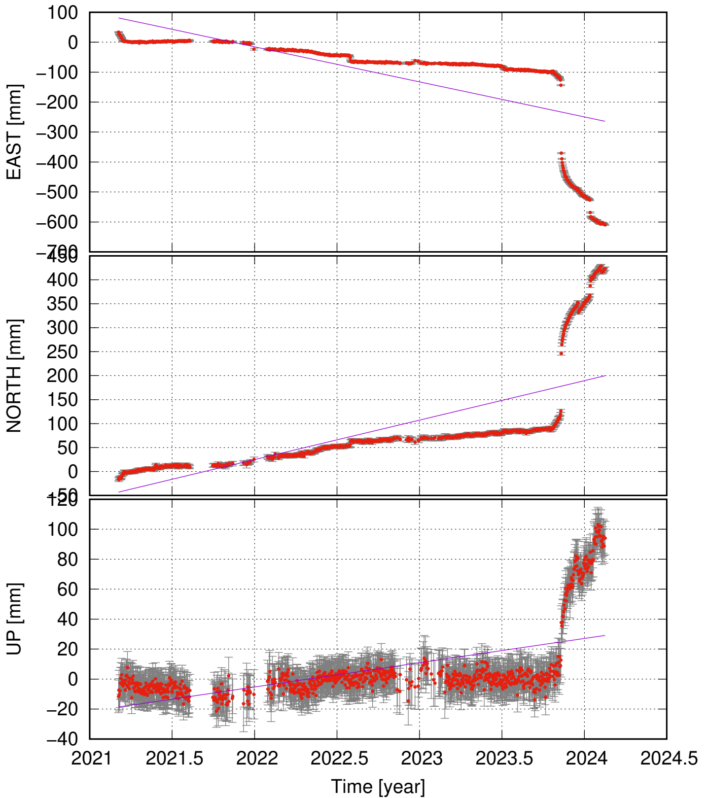
NAMC (63.92, -22.54) time series (ITRF 2014) v_e = -116.97 \pm 38.49 ; v_n = 82.30 \pm 24.13 ; v_u = 16.18 \pm 6.98 mm/yr
