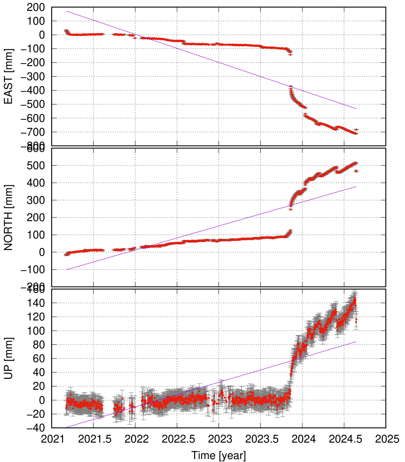
NAMC (63.92, -22.54) time series (ITRF 2014) v_e = -202.87 \pm 43.72 ; v_n = 138.33 \pm 28.29 ; v_u = 35.62 \pm 8.96 mm/yr
