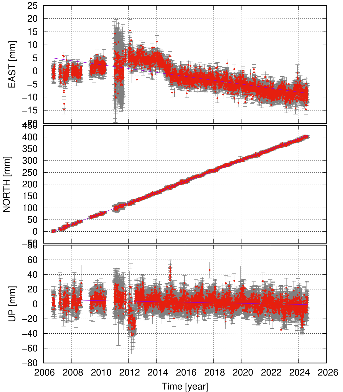
MYVA (65.64, -16.89) time series (ITRF 2014) v_e = -0.75 \pm 0.16 ; v_n = 22.71 \pm 0.17 ; v_u = -0.37 \pm 0.46 mm/yr
