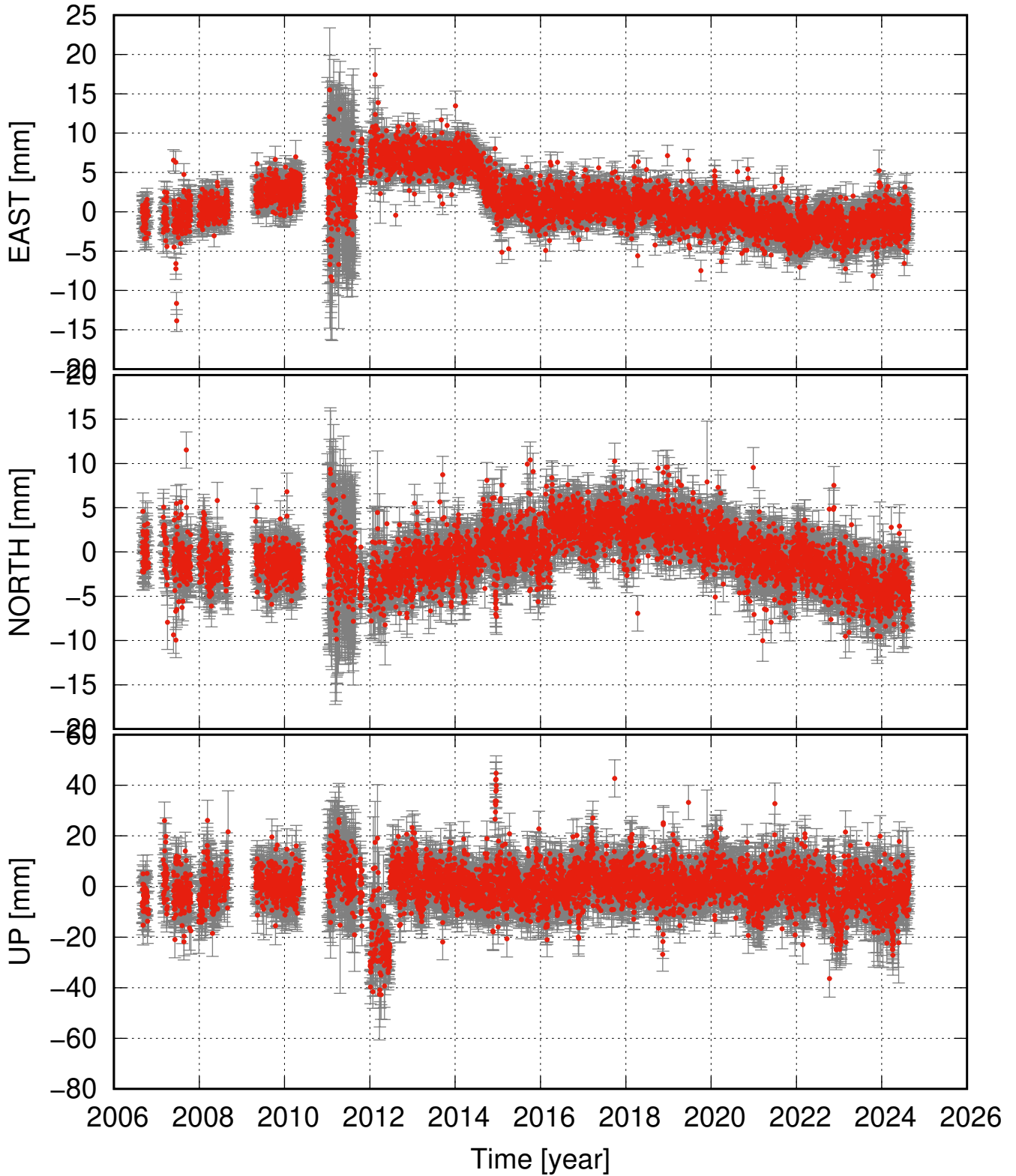
MYVA detrended and seasonal signal removed
