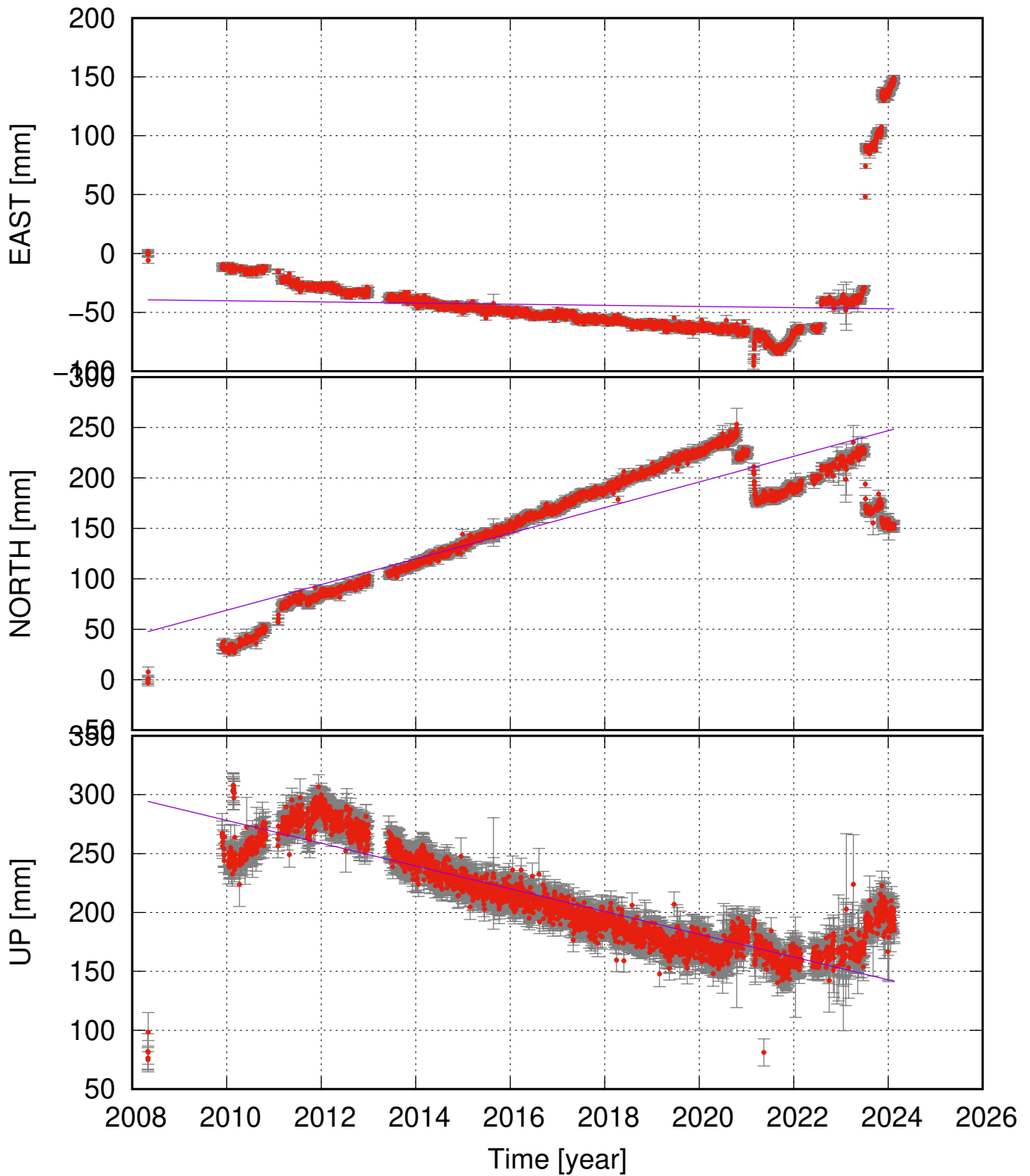
MOHA (63.92, -22.06) time series (ITRF 2014) v_e = -0.47 \pm 2.40 ; v_n = 12.70 \pm 1.69 ; v_u = -9.66 \pm 1.20 mm/yr
