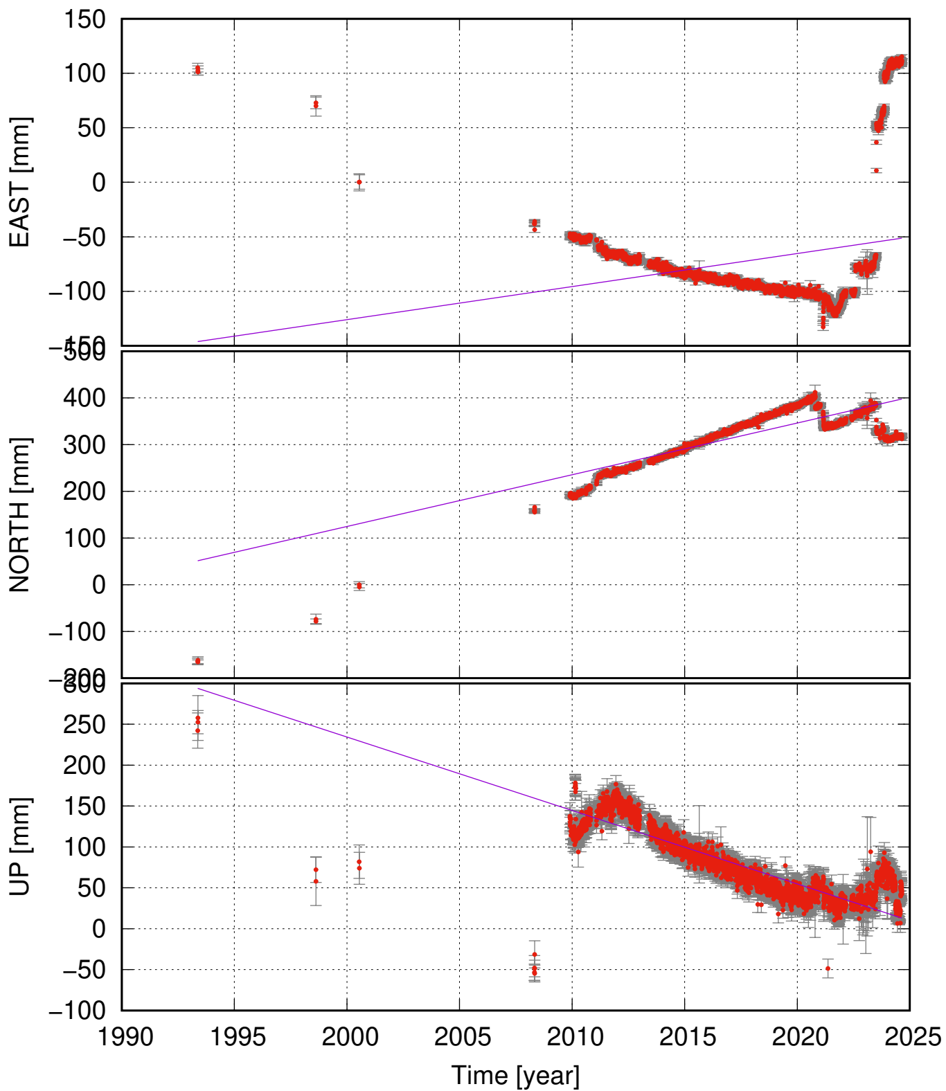
MOHA (63.92, -22.06) time series (ITRF 2014) v_e = 3.03 \pm 1.67 ; v_n = 11.08 \pm 1.03 ; v_u = -8.97 \pm 0.65 mm/yr
