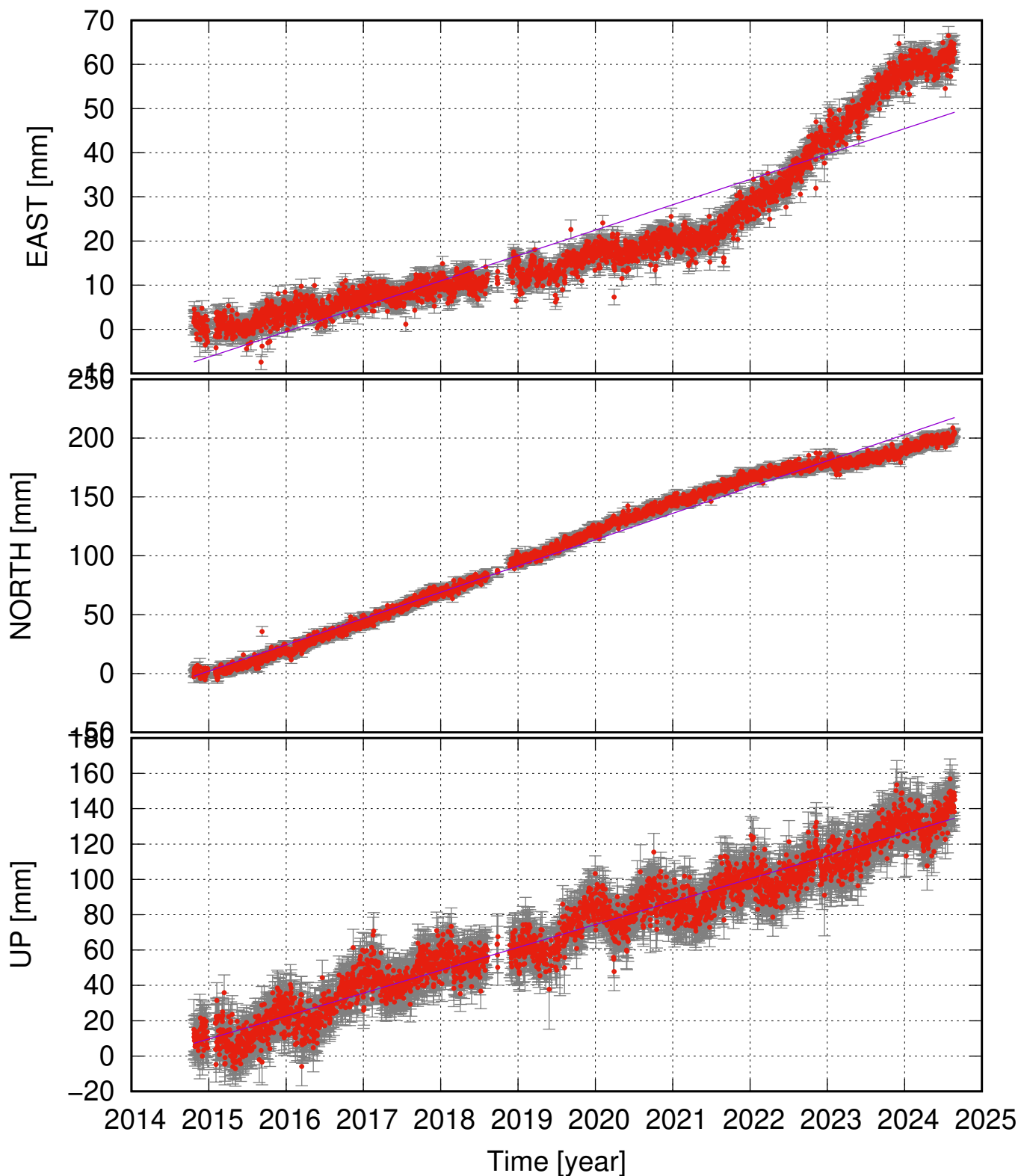
MOFC (64.98, -16.67) time series (ITRF 2014) v_e = 5.75 \pm 0.70 ; v_n = 22.33 \pm 0.75 ; v_u = 12.95 \pm 0.83 mm/yr
