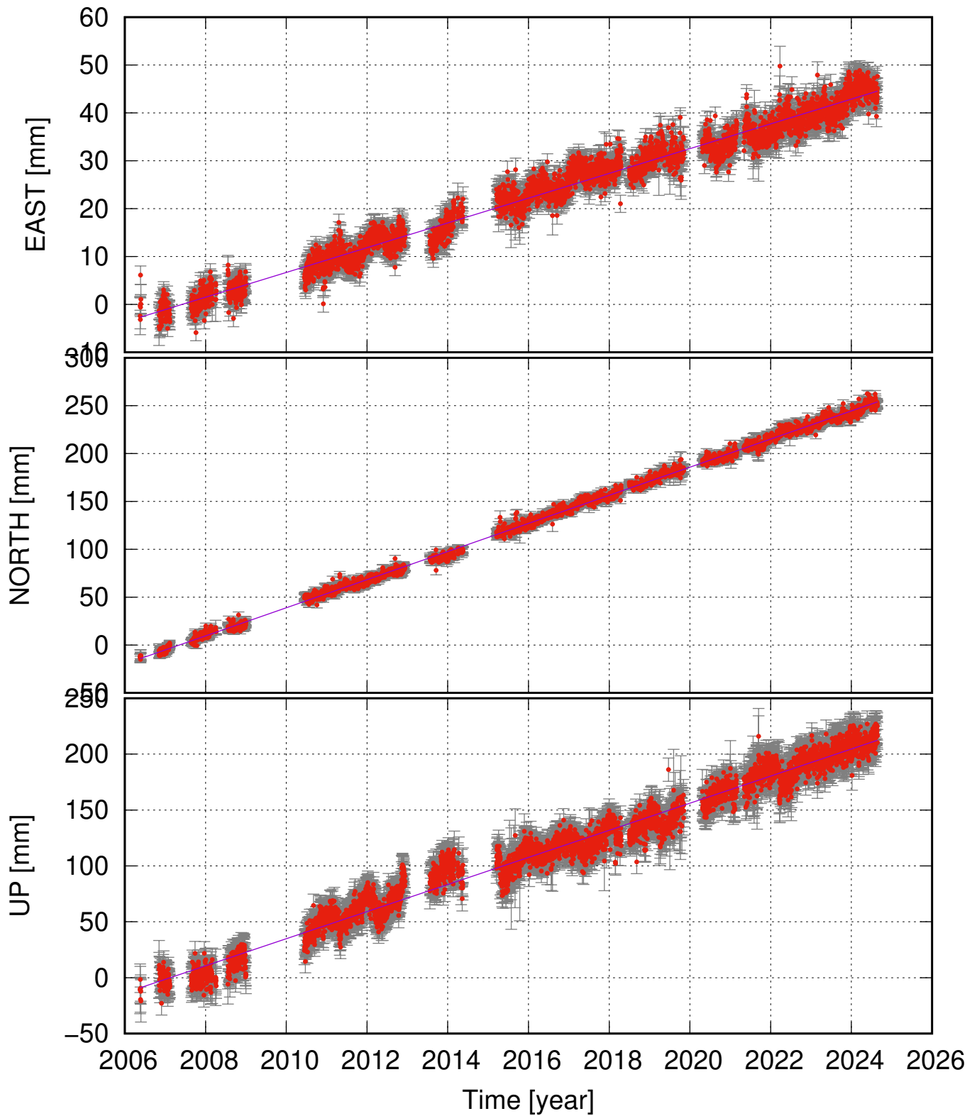
MJSK (63.93, -19.67) time series (ITRF 2014) v_e = 2.59 \pm 0.11 ; v_n = 14.68 \pm 0.17 ; v_u = 12.12 \pm 0.51 mm/yr
