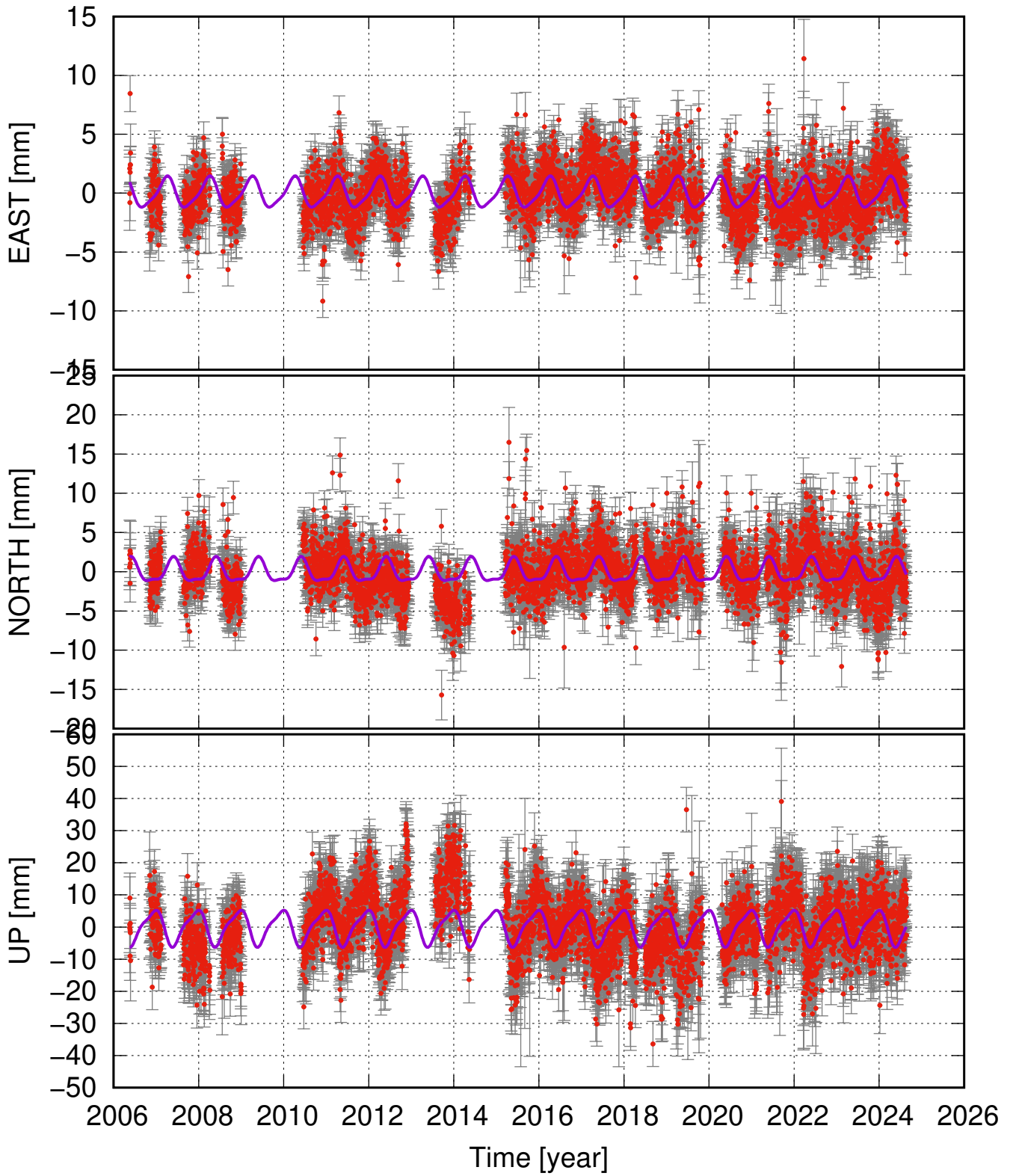
MJSK seasonal fit
