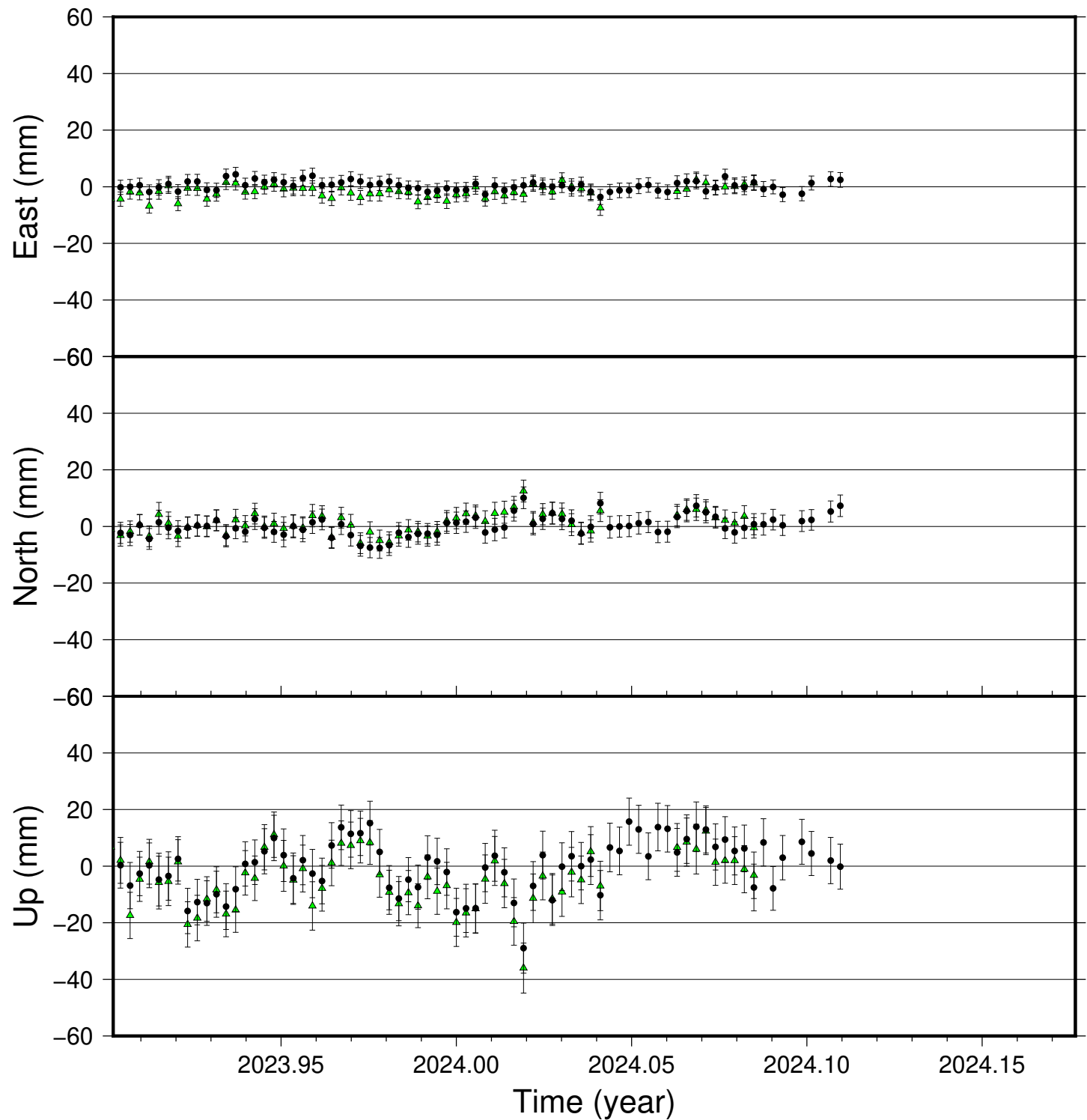
MJSK time series (IGS 2014), last 100 days
