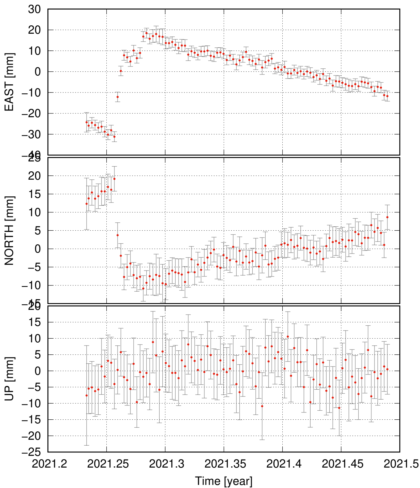
MERC residual time series (some major events removed as well)
