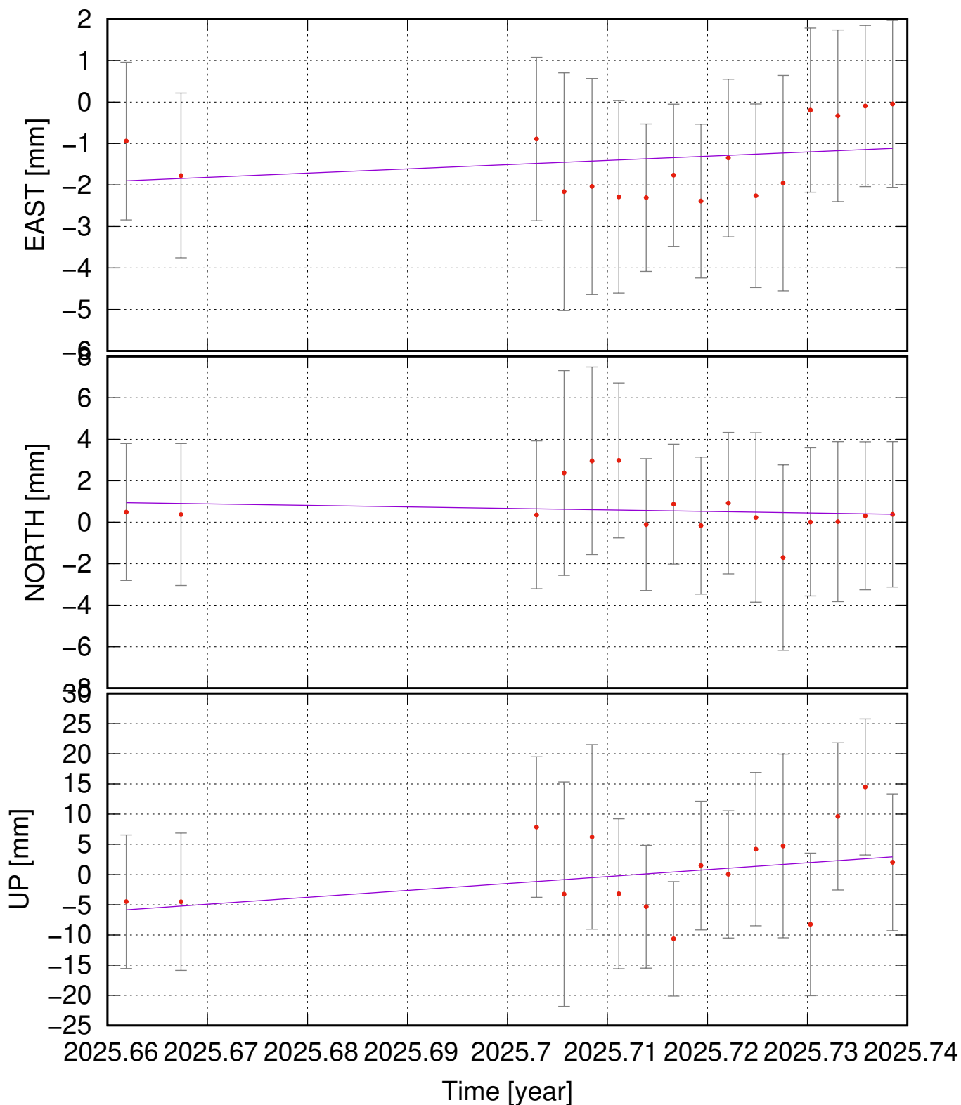
MANC (66.30, -17.12) time series (IGb20) v_e = 10.20 \pm 11.38 ; v_n = -7.30 \pm 16.07 ; v_u = 114.60 \pm 86.49 mm/yr
