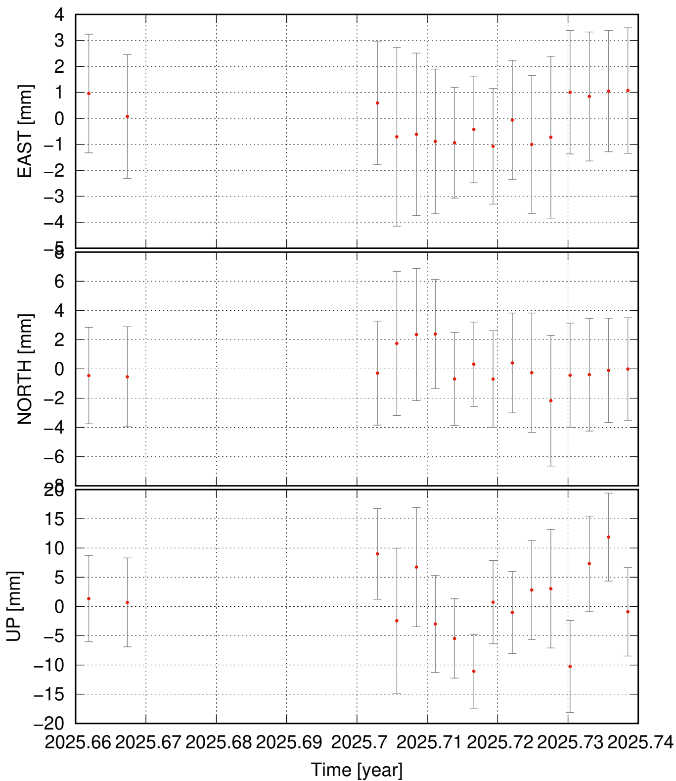
MANC residual time series (some major events removed as well)
