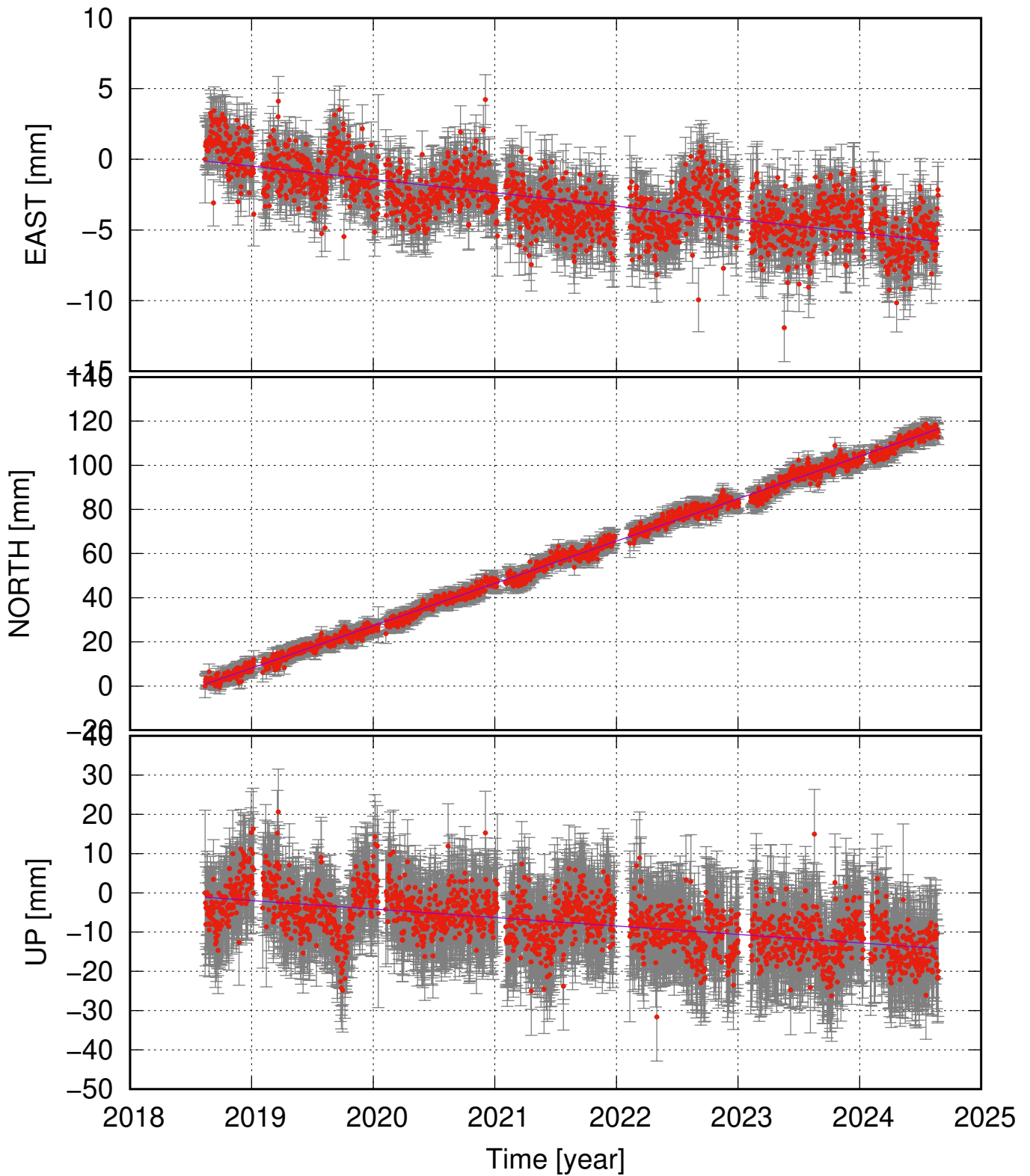
MANA (66.30, -17.12) time series (ITRF 2014) v_e = -0.95 \pm 0.26 ; v_n = 19.17 \pm 0.32 ; v_u = -2.15 \pm 0.91 mm/yr
