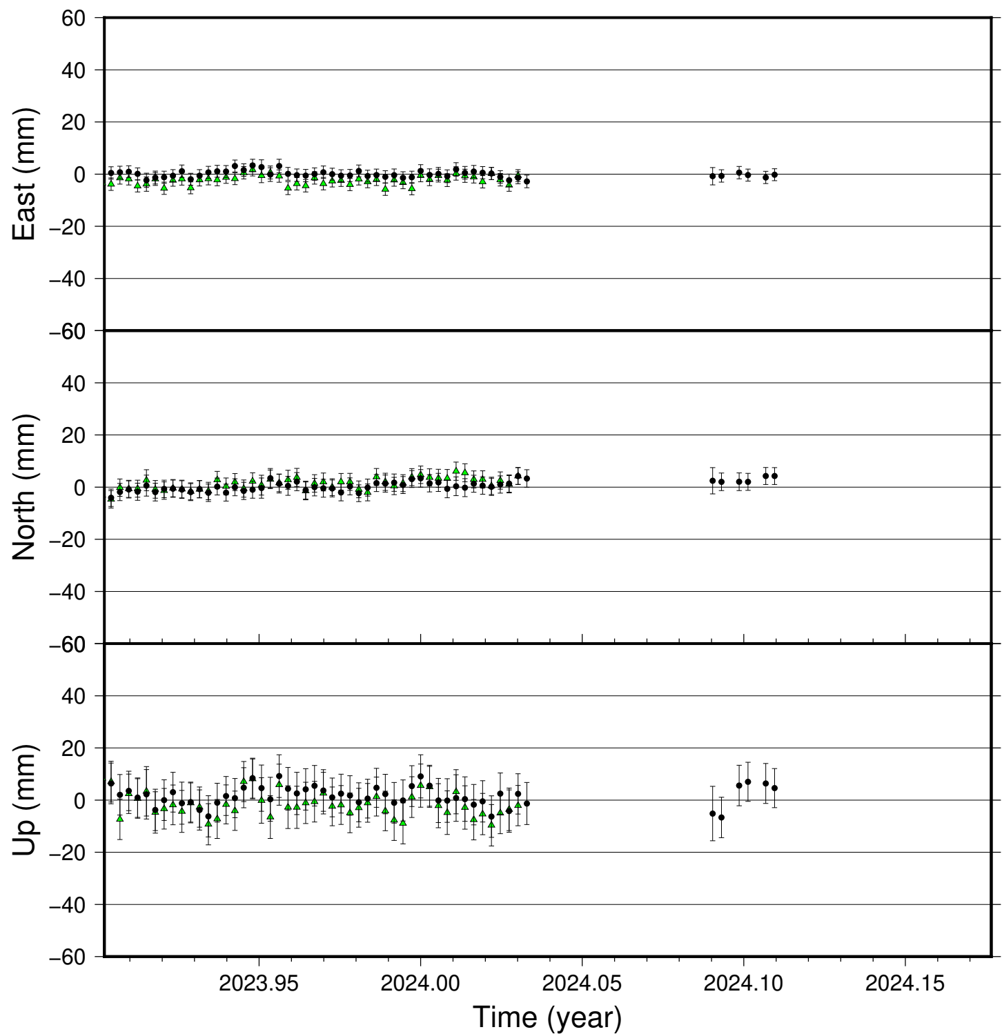
MANA time series (IGS 2014), last 100 days
