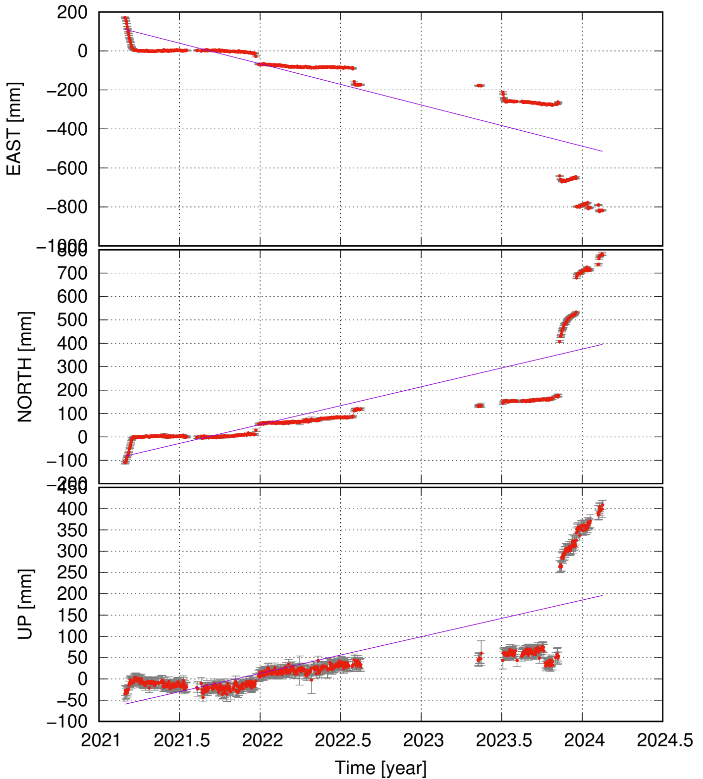
LSK (63.92, -22.37) time series (ITRF 2014) ve = -211.32 ± 39.72; vn = 161.35 ± 39.52; vu = 86.12 ± 23.63 mm/yr
