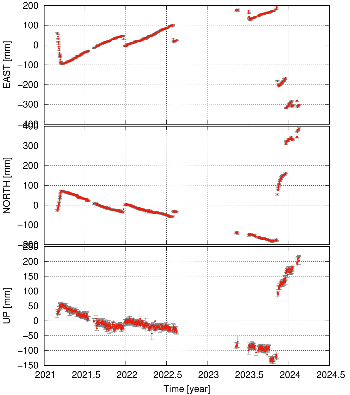
LISK residual time series (some major events removed as well)
