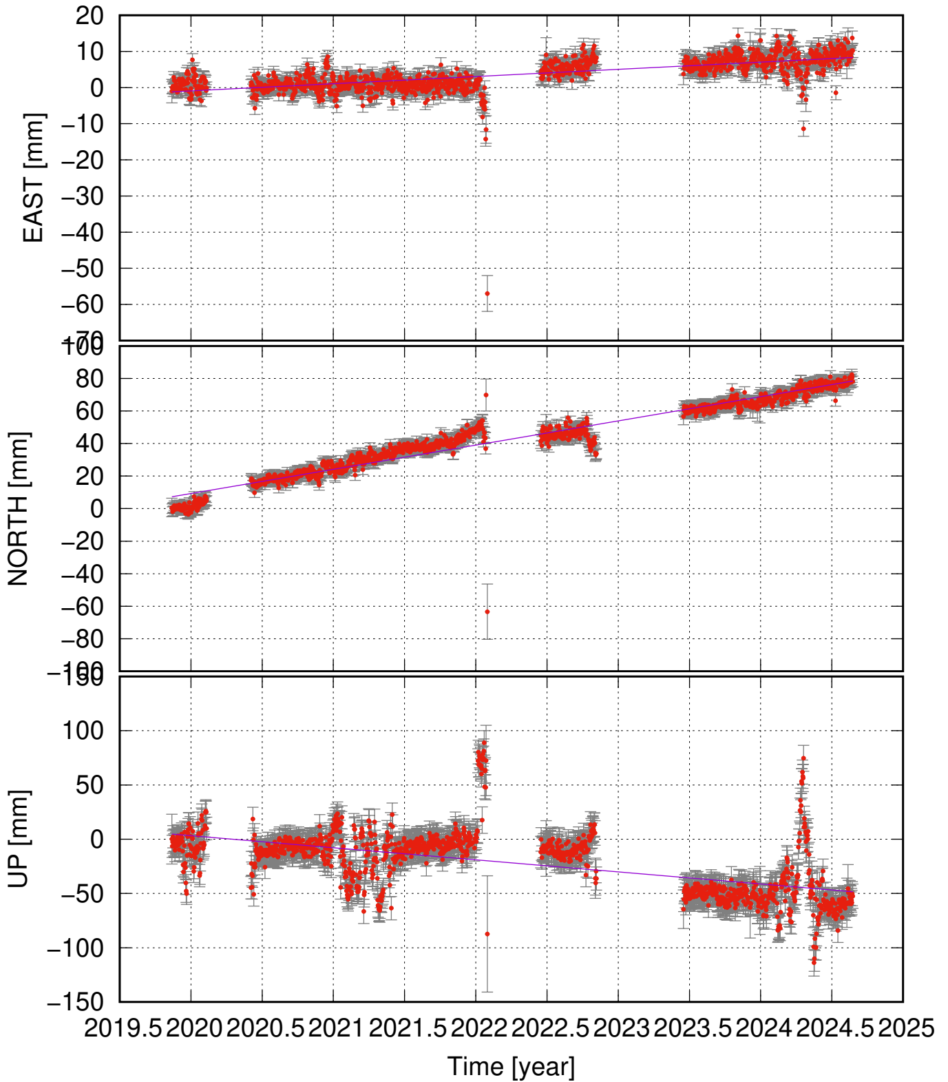
LHNC (65.72, -16.78) time series (ITRF 2014) v_e = 1.99 \pm 0.66 ; v_n = 14.88 \pm 1.15 ; v_u = -11.12 \pm 4.80 mm/yr
