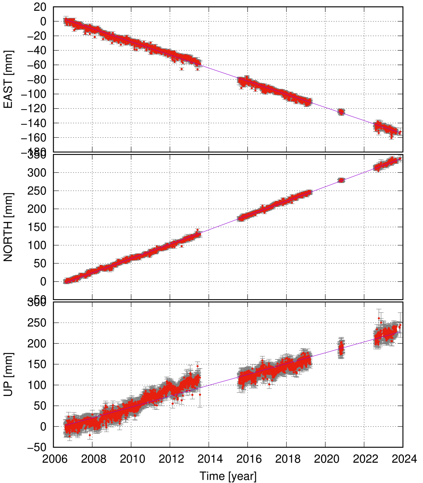
LFEL (64.53, -19.76) time series (ITRF 2014) v_e = -9.04 \pm 0.13 ; v_n = 19.77 \pm 0.17 ; v_u = 13.07 \pm 0.68 mm/yr
