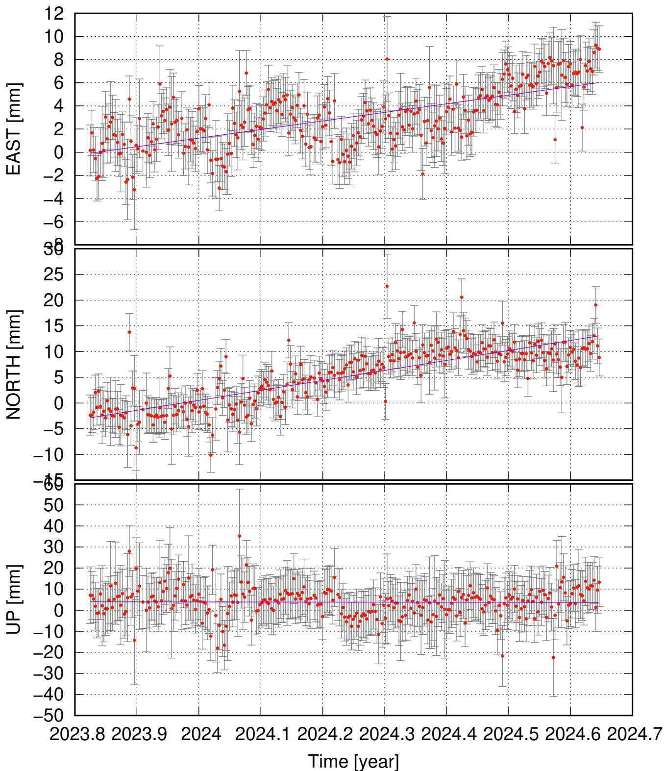
LAVI (64.83, -13.83) time series (ITRF 2014) ve = 7.42 \pm 2.32 ; vn = 19.39 \pm 3.88 ; vu = -0.40 \pm 8.27 mm/yr
