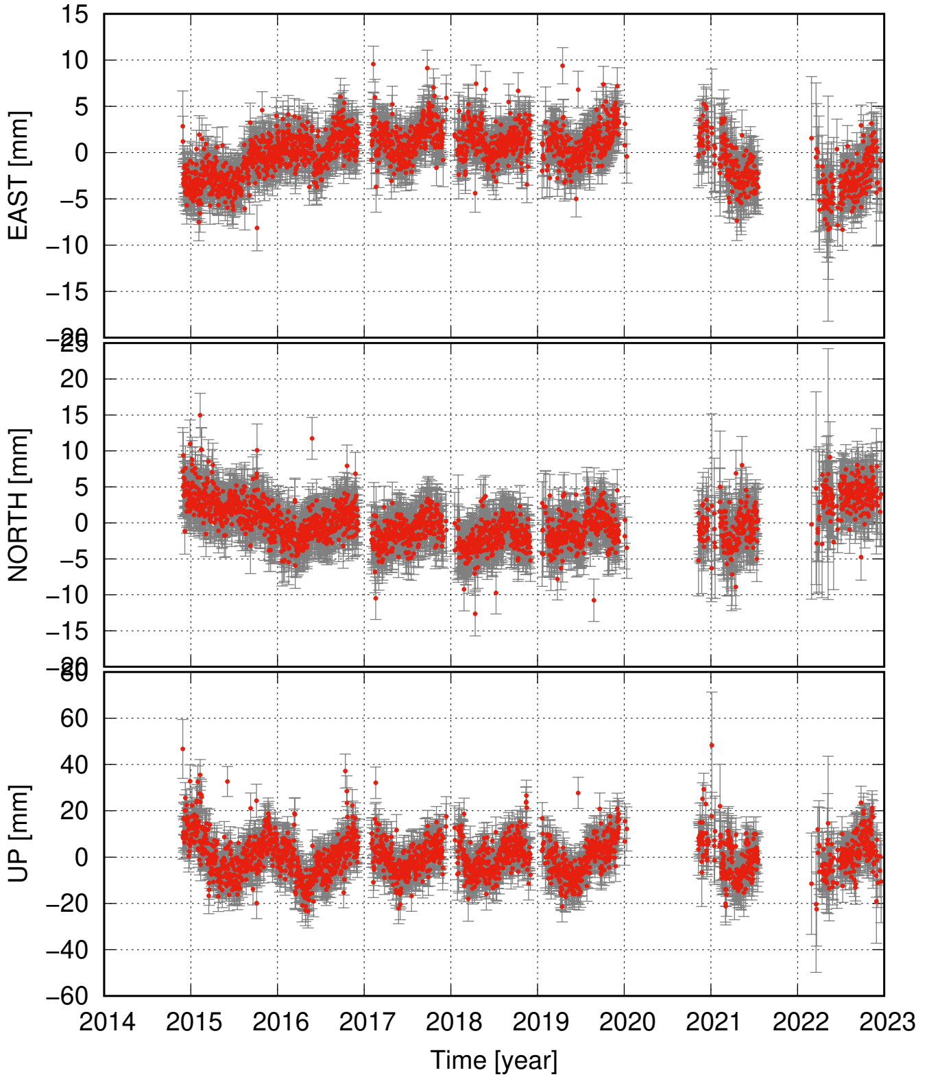
LANH residual time series (some major events removed as well)
