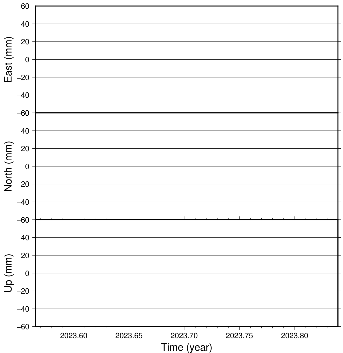
LANH time series (IGS 2014), last 100 days
