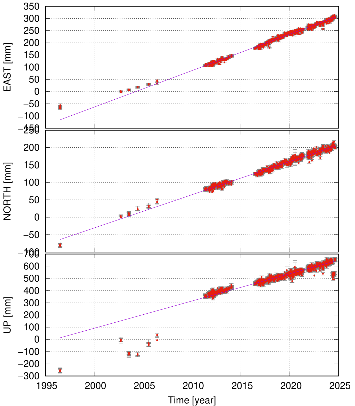
KVSK (63.98, -16.43) time series (ITRF 2014) v_e = 14.95 \pm 0.17 ; v_n = 9.54 \pm 0.13 ; v_u = 22.35 \pm 1.23 mm/yr
