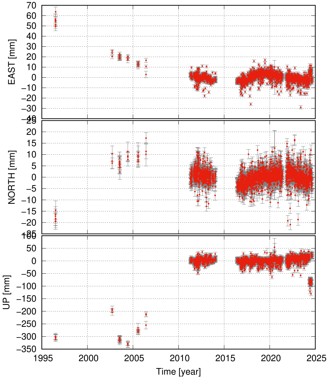
KVSK detrended and seasonal signal removed
