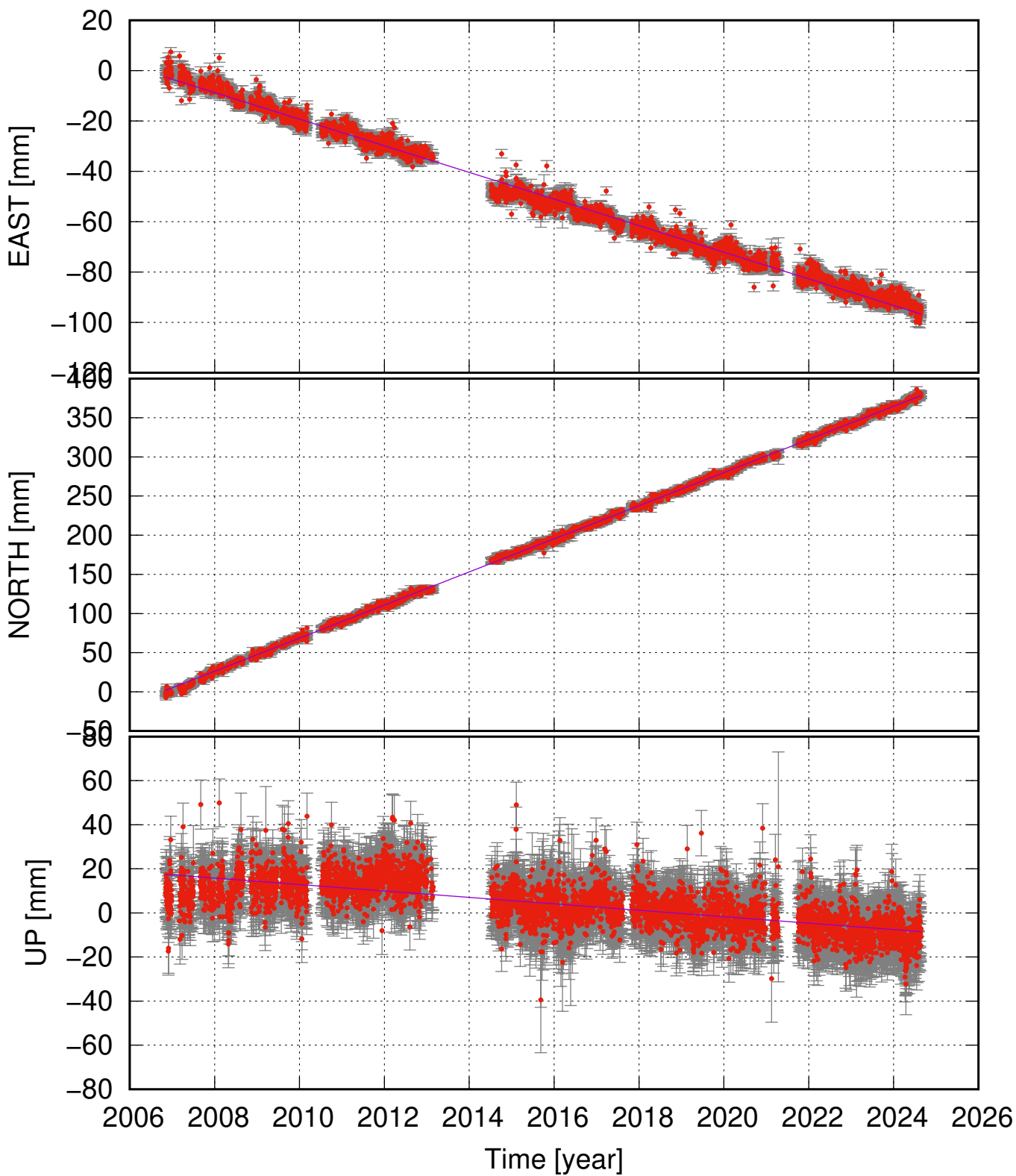
KVIS (66.10, -17.27) time series (ITRF 2014) v_e = -5.28 \pm 0.14 ; v_n = 21.15 \pm 0.13 ; v_u = -1.46 \pm 0.41 mm/yr
