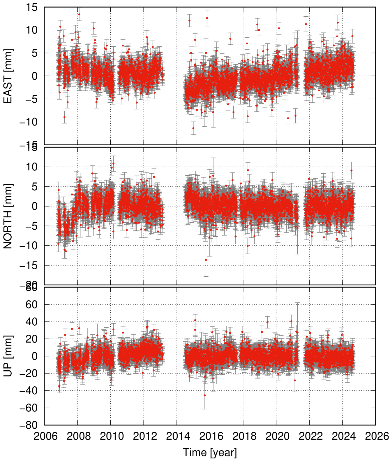
KVIS detrended and seasonal signal removed
