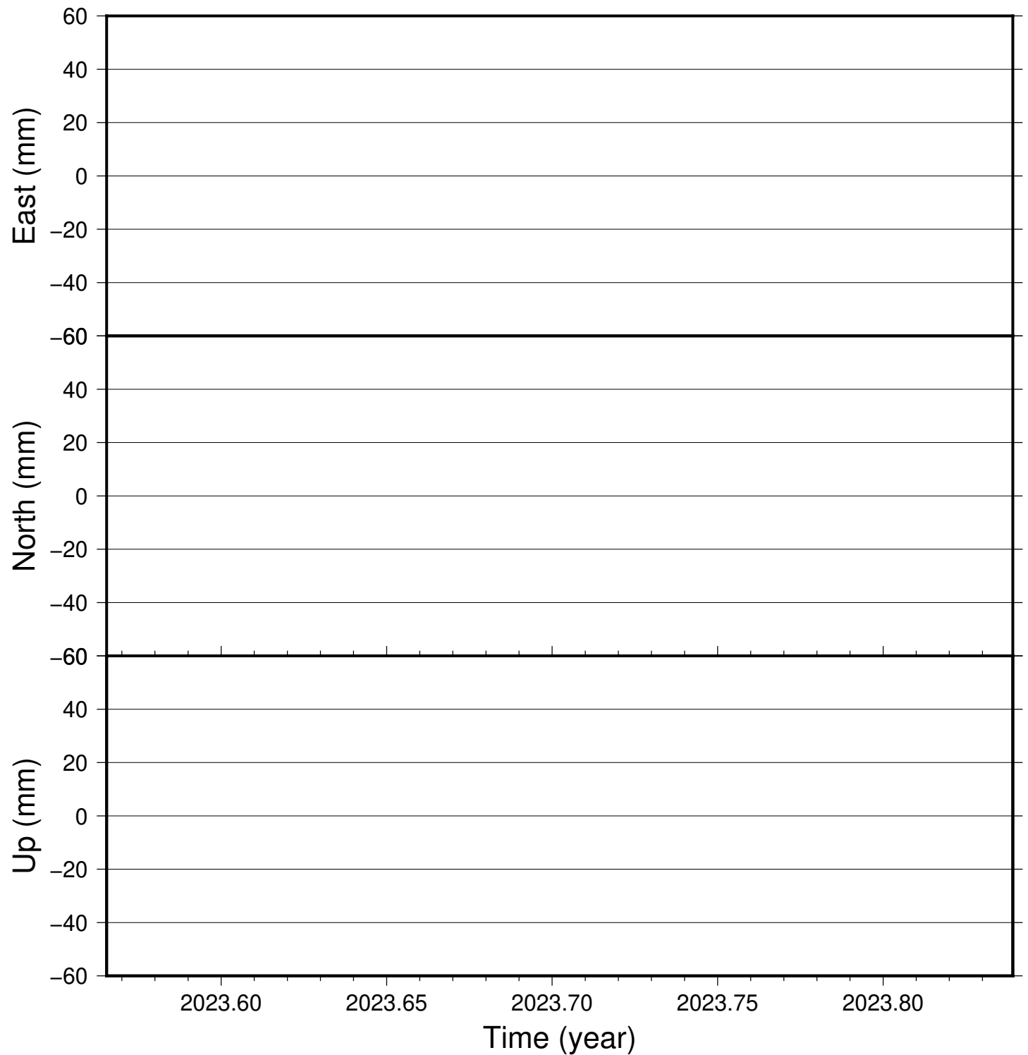
KVIC time series (IGS 2014), last 100 days
