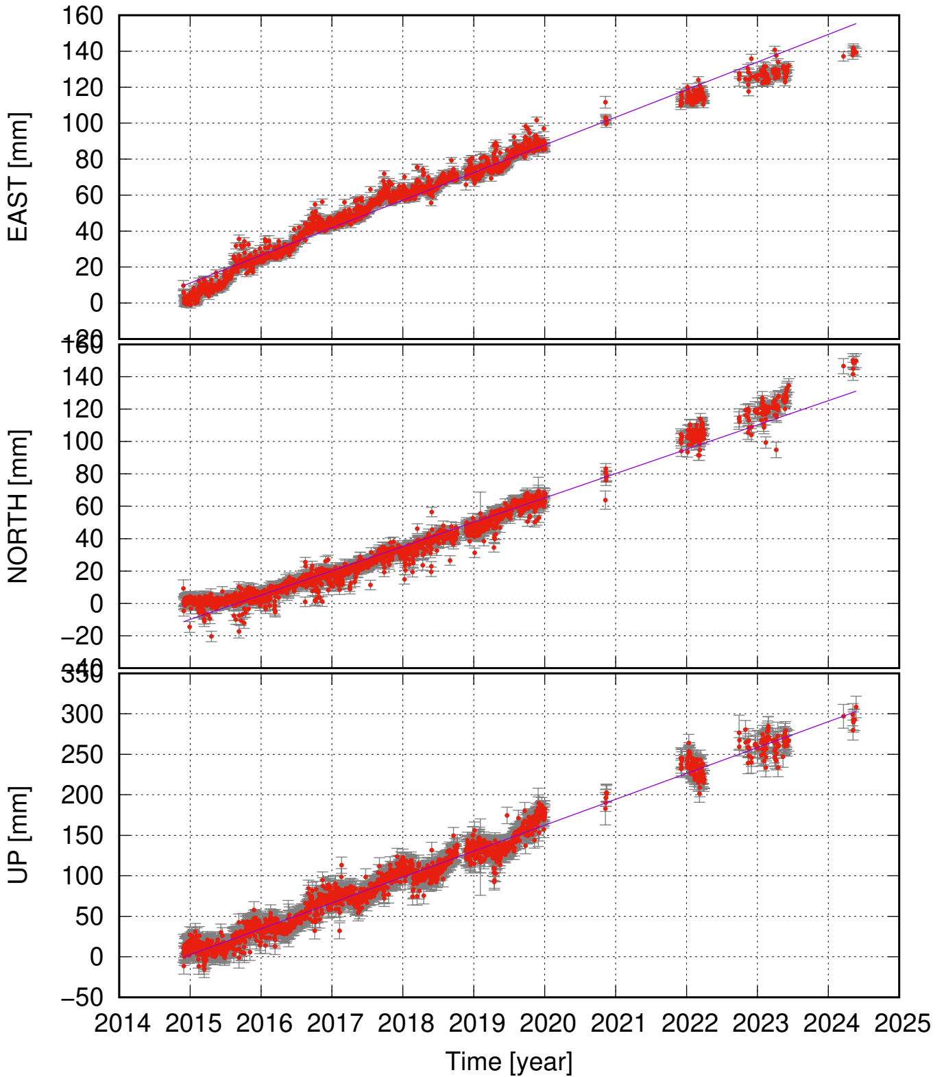
KVEC (64.75, -16.65) time series (ITRF 2014) v_e = 15.35 \pm 0.53 ; v_n = 15.01 \pm 0.57 ; v_u = 31.95 \pm 1.06 mm/yr
