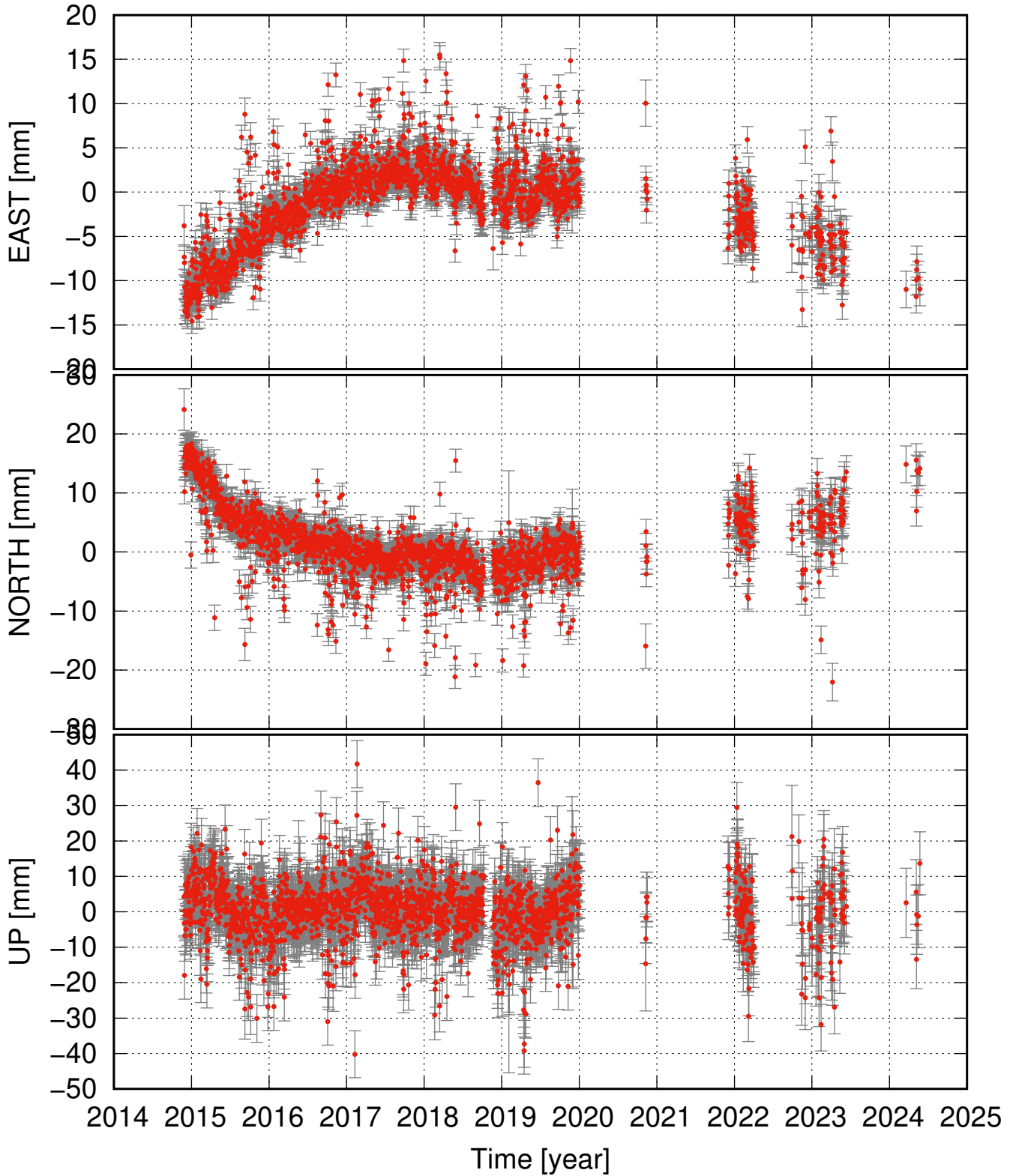
KVEC detrended and seasonal signal removed
