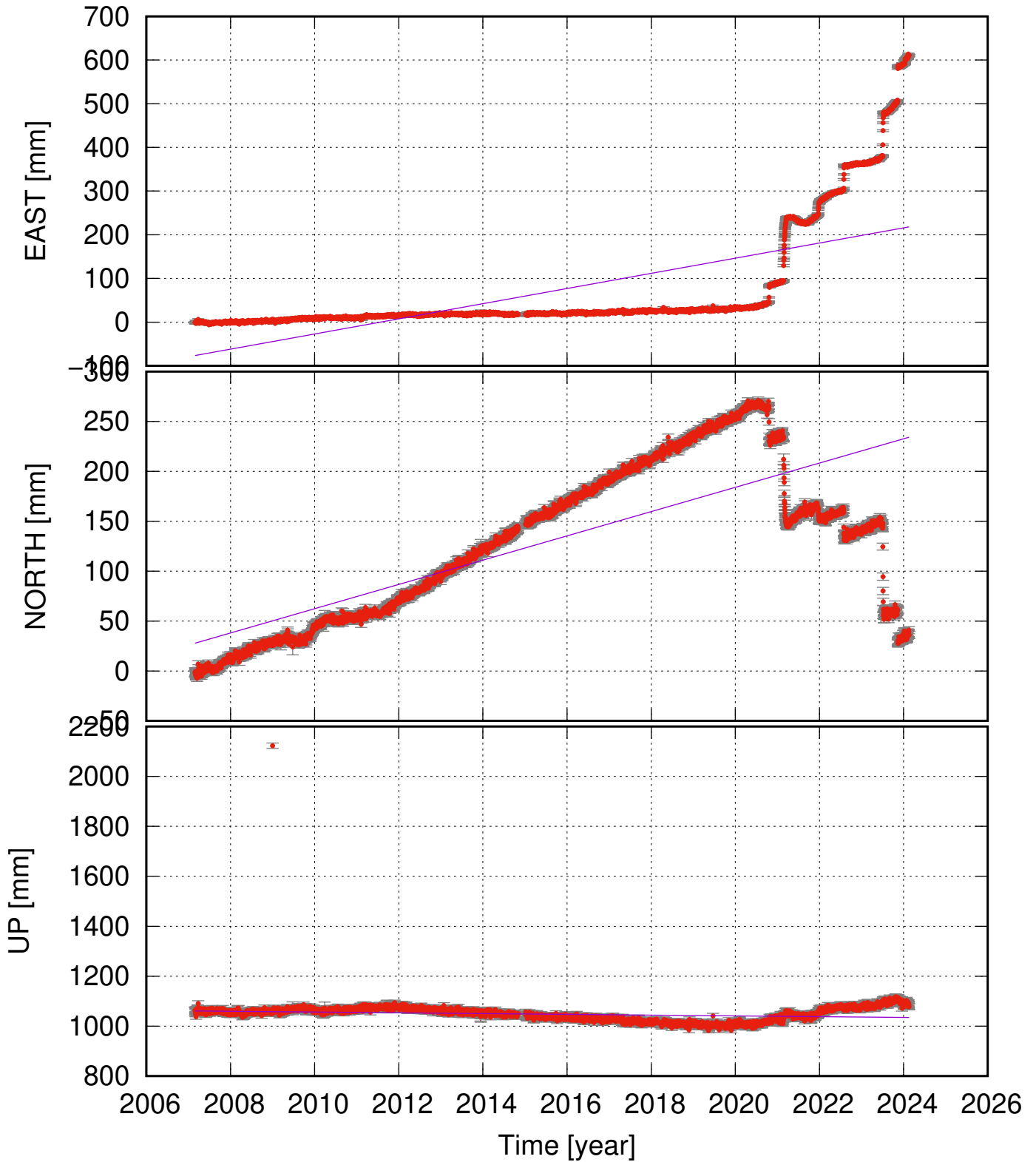
KRIV (63.88, -22.08) time series (ITRF 2014) v_e = 17.36 \pm 5.77 ; v_n = 12.16 \pm 3.27 ; v_u = -1.58 \pm 1.68 mm/yr
