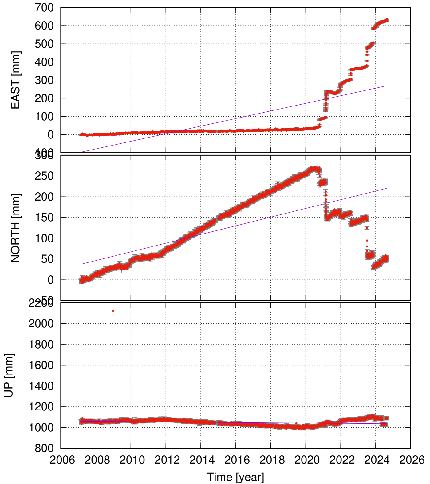
KRIV (63.88, -22.08) time series (ITRF 2014) v_e = 20.89 \pm 6.57 ; v_n = 10.46 \pm 3.57 ; v_u = -1.32 \pm 1.65 mm/yr
