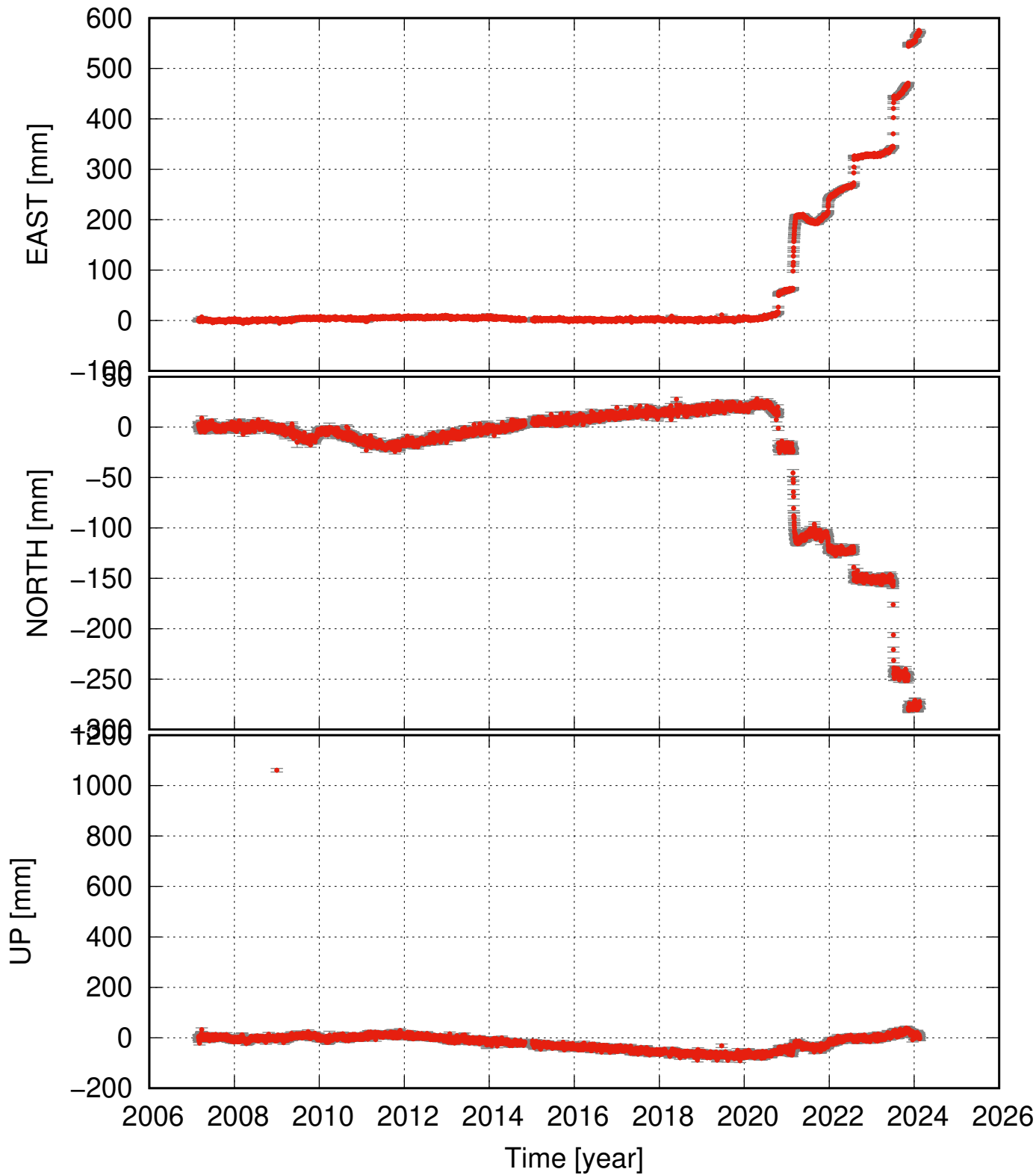
KRIV detrended and seasonal signal removed
