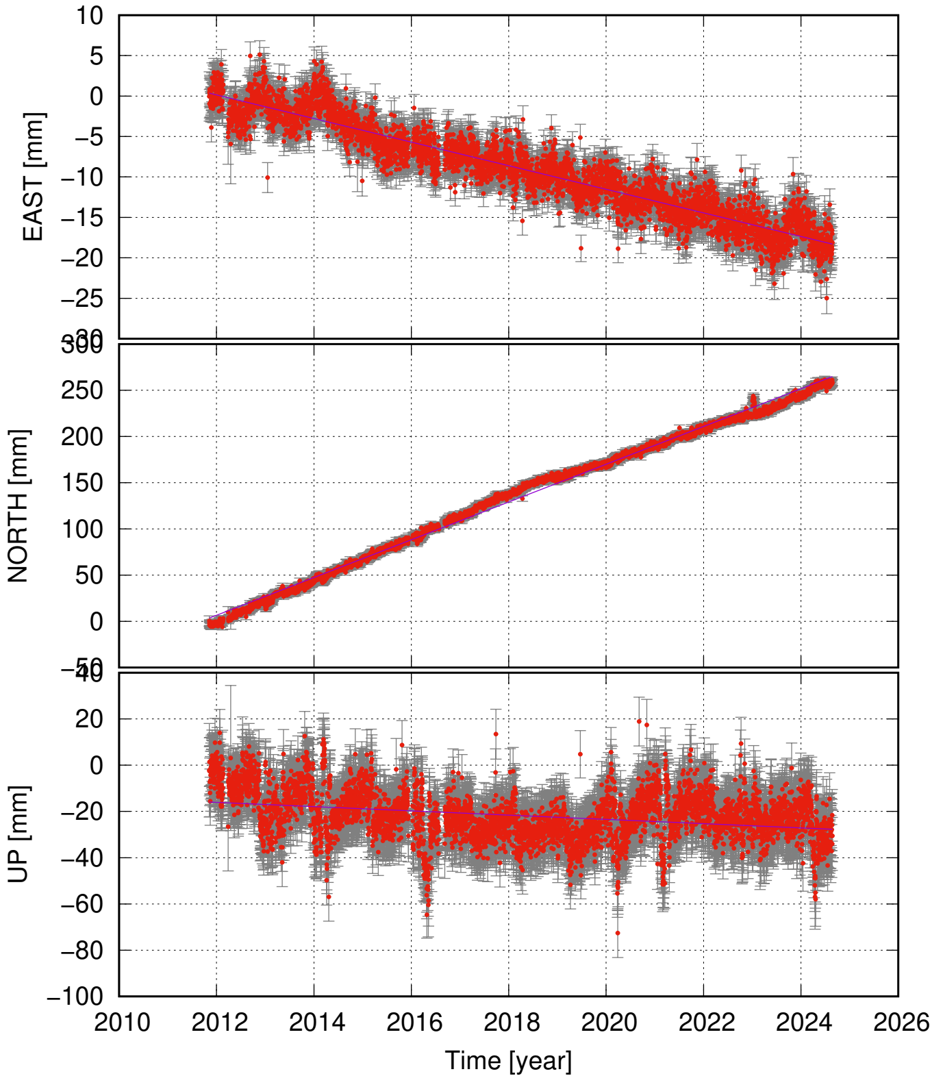
KRAC (65.69, -16.77) time series (ITRF 2014) v_e = -1.46 \pm 0.14 ; v_n = 20.42 \pm 0.44 ; v_u = -0.92 \pm 0.76 mm/yr
